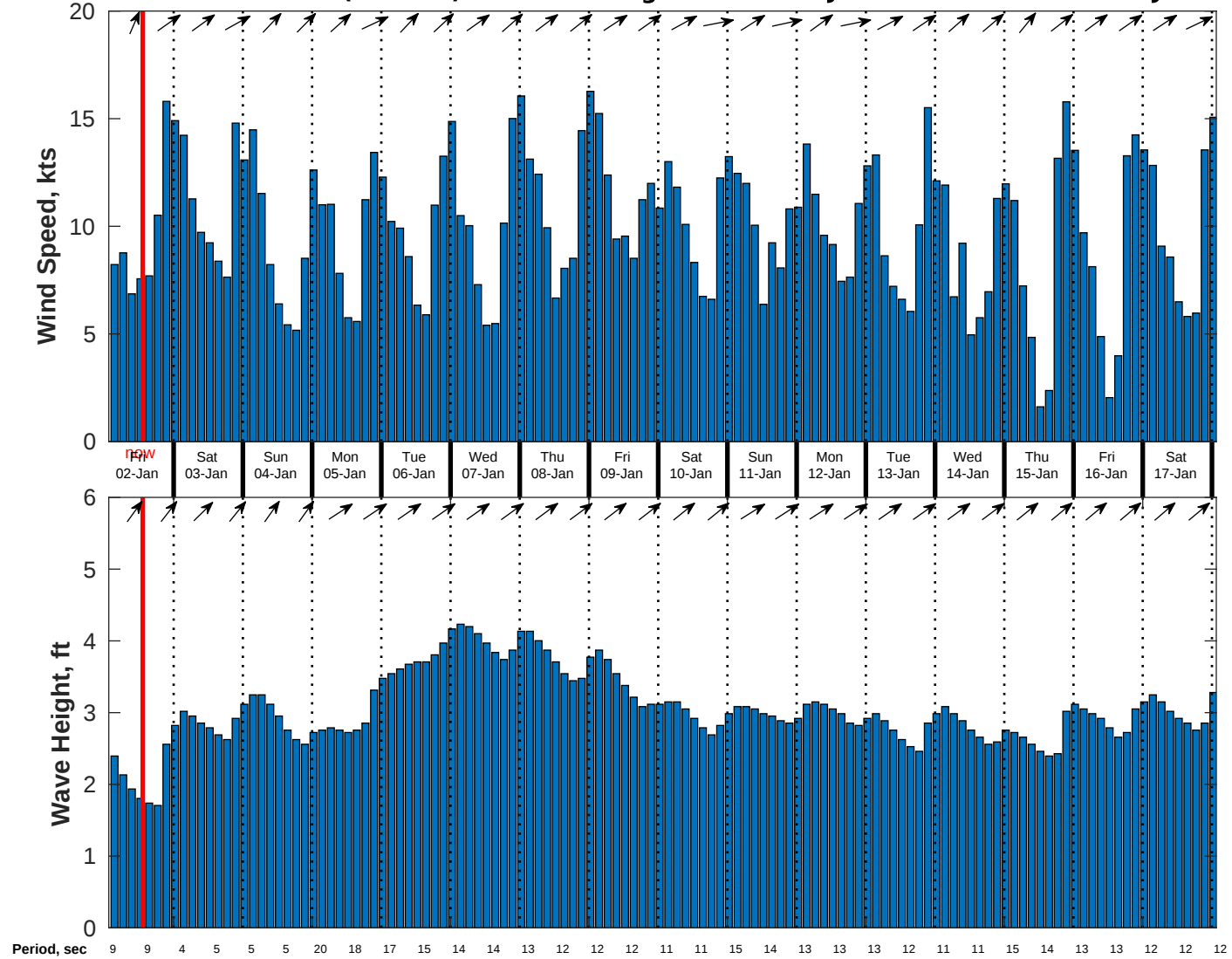
Wind & Wave Forecast for CSA (ONHYM) PPL EBS - Nigeria from 01-Jan-2026 02:00:00 to 17-Jan-2026 02:00:00
