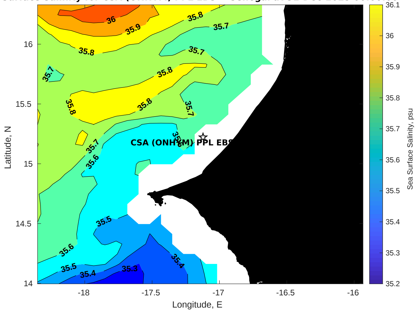
Surface Salinity for CSA (ONHYM) PPL EBS - Senegal at 31-Dec-2025 00:00:00
