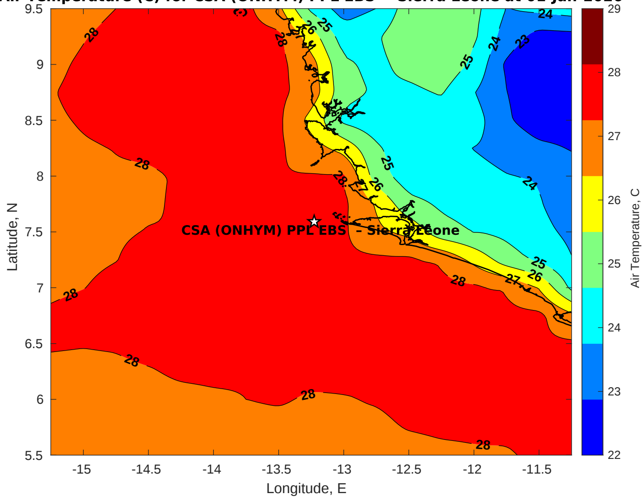
Air Temperature (C) for CSA (ONHYM) PPL EBS - Sierra Leone at 01-Jan-2026
