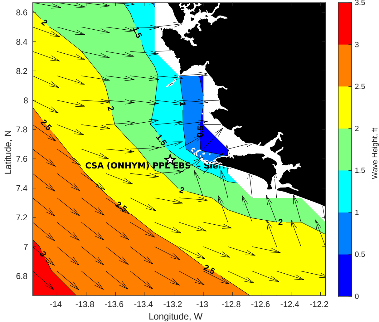
GFS Wave Height (ft) for CSA (ONHYM) PPL EBS - Sierra Leone at 01-Jan-2026 09:00:00
