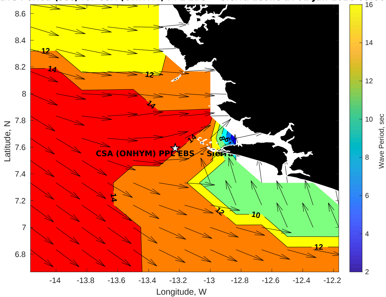
GFS Wave Period (sec) for CSA (ONHYM) PPL EBS - Sierra Leone at 01-Jan-2026 09:00:00
