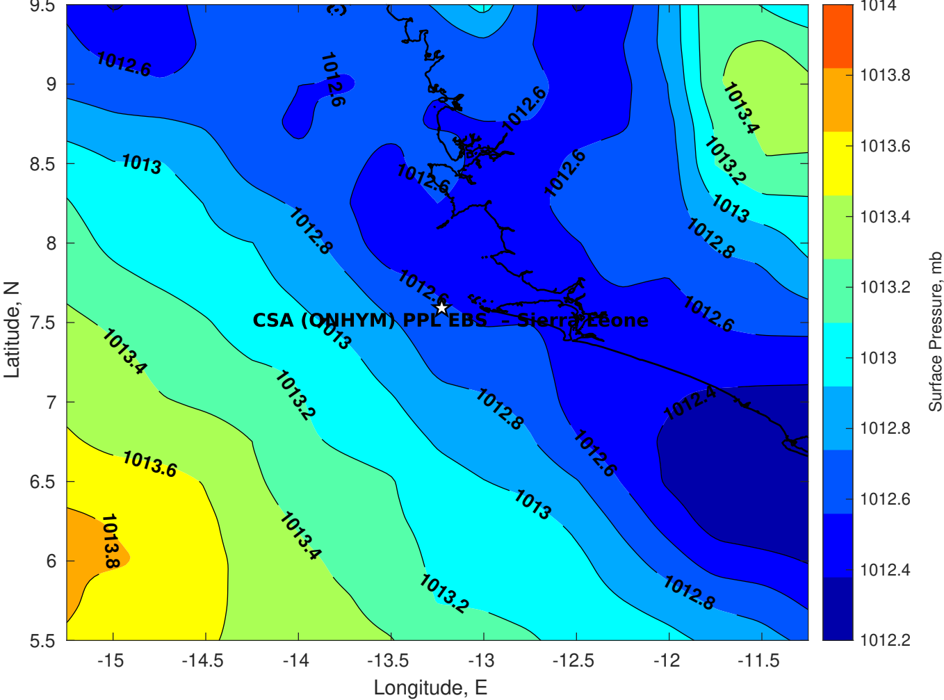
Surface Pressure (mb) for CSA (ONHYM) PPL EBS - Sierra Leone at 02-Jan-2026 00:00:00
