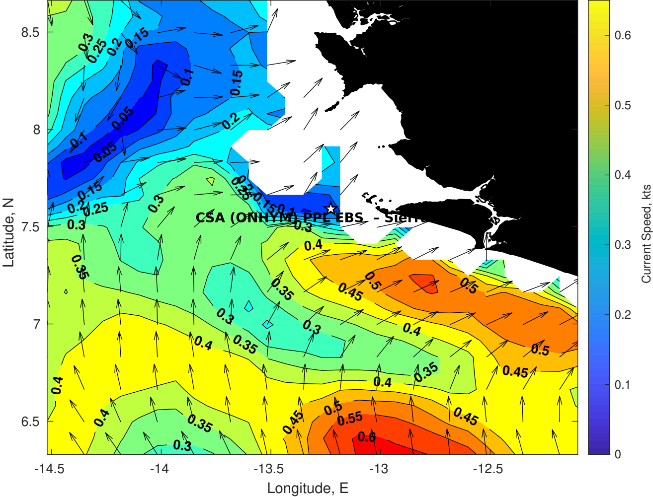
Surface Currents for CSA (ONHYM) PPL EBS - Sierra Leone at 31-Dec-2025 00:00:00
