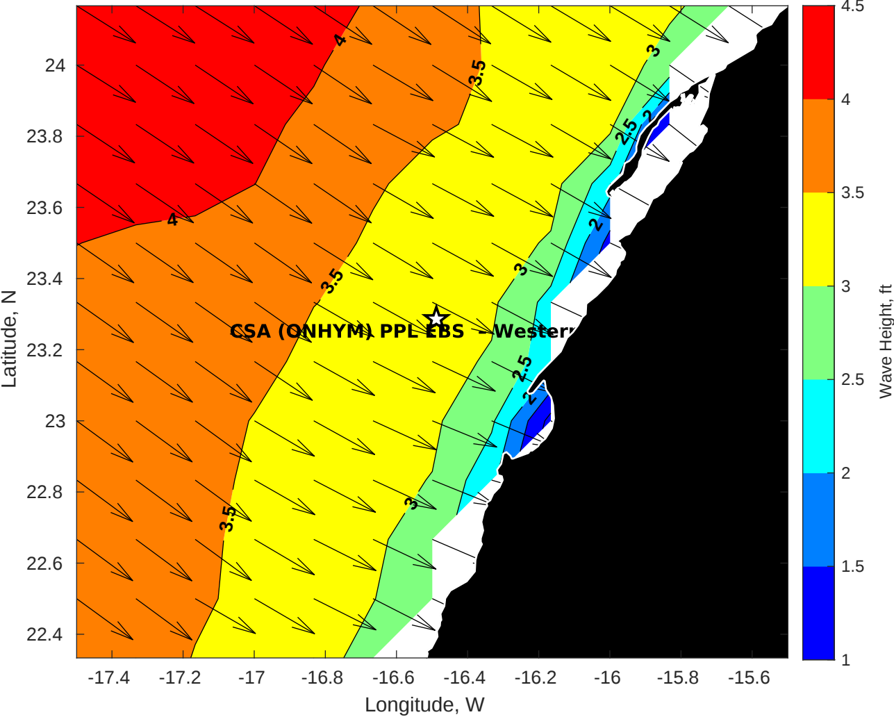
GFS Wave Height (ft) for CSA (ONHYM) PPL EBS - Western Sahara at 01-Jan-2026 09:00:00
