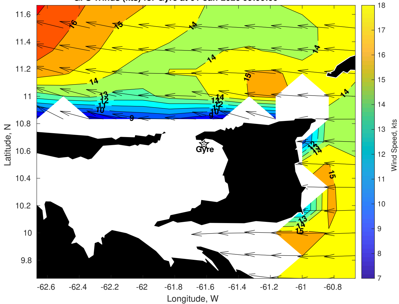
GFS Winds (kts) for Gyre at 01-Jan-2026 09:00:00
