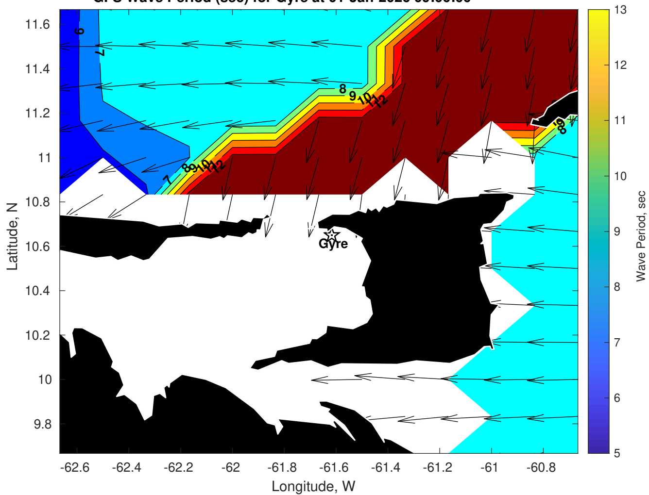
GFS Wave Period (sec) for Gyre at 01-Jan-2026 09:00:00
