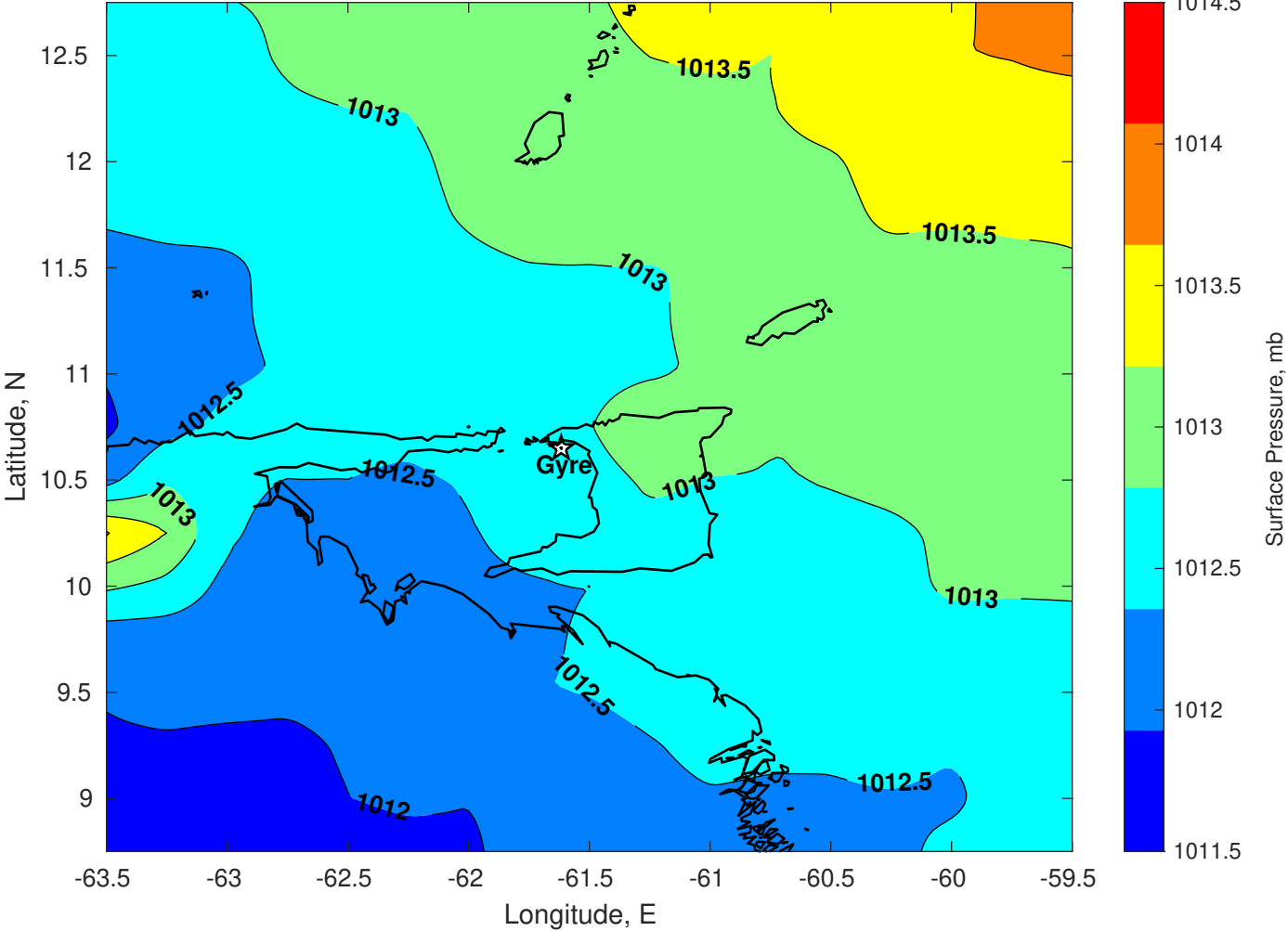
Surface Pressure (mb) for Gyre at 03-Jan-2026 00:00:00
