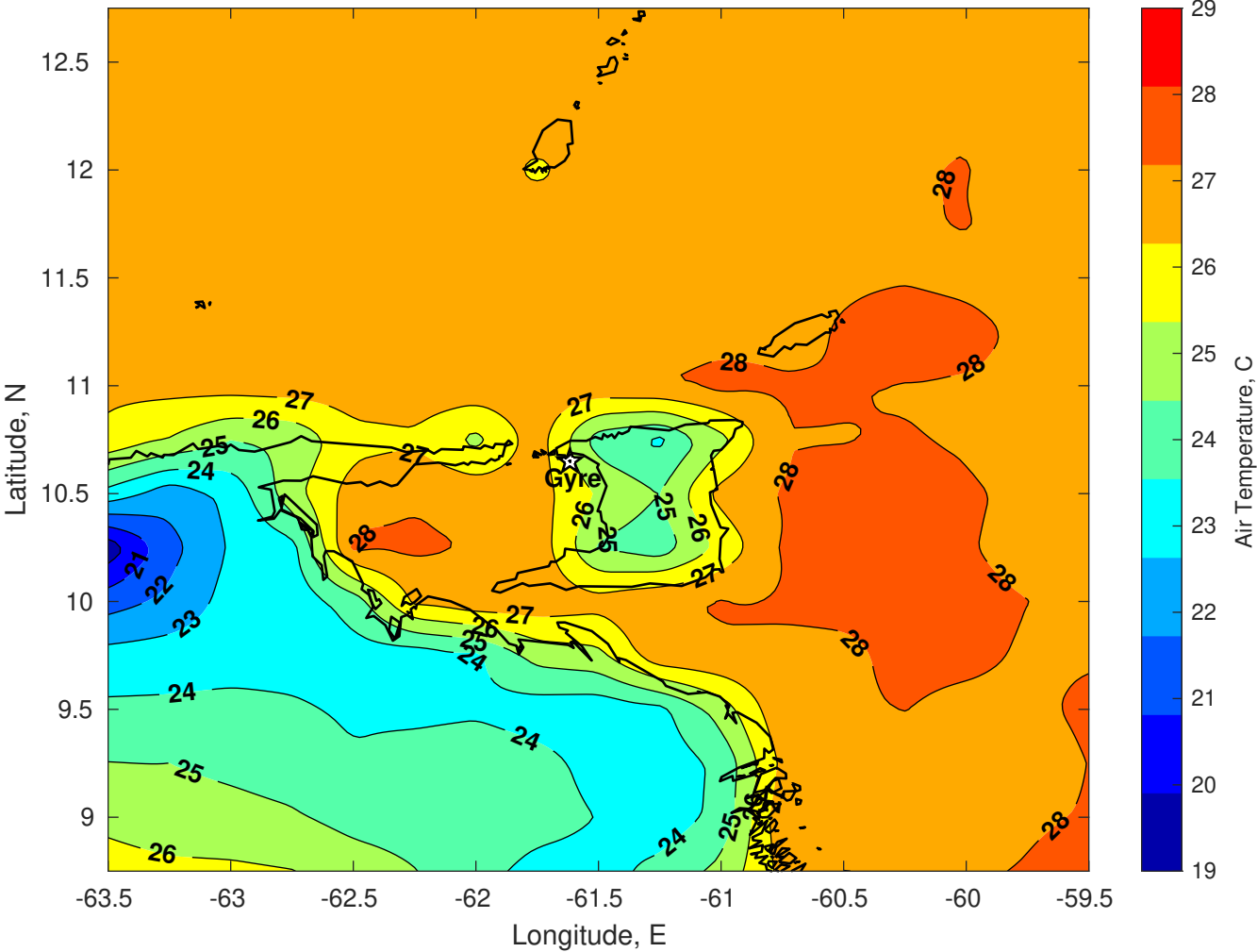
Air Temperature (C) for Gyre at 01-Jan-2026
