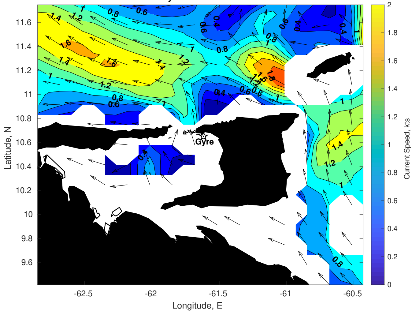
Surface Currents for Gyre at 31-Dec-2025 00:00:00
