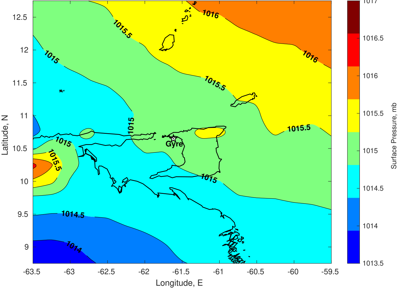
Surface Pressure (mb) for Gyre at 01-Jan-2026 00:00:00
