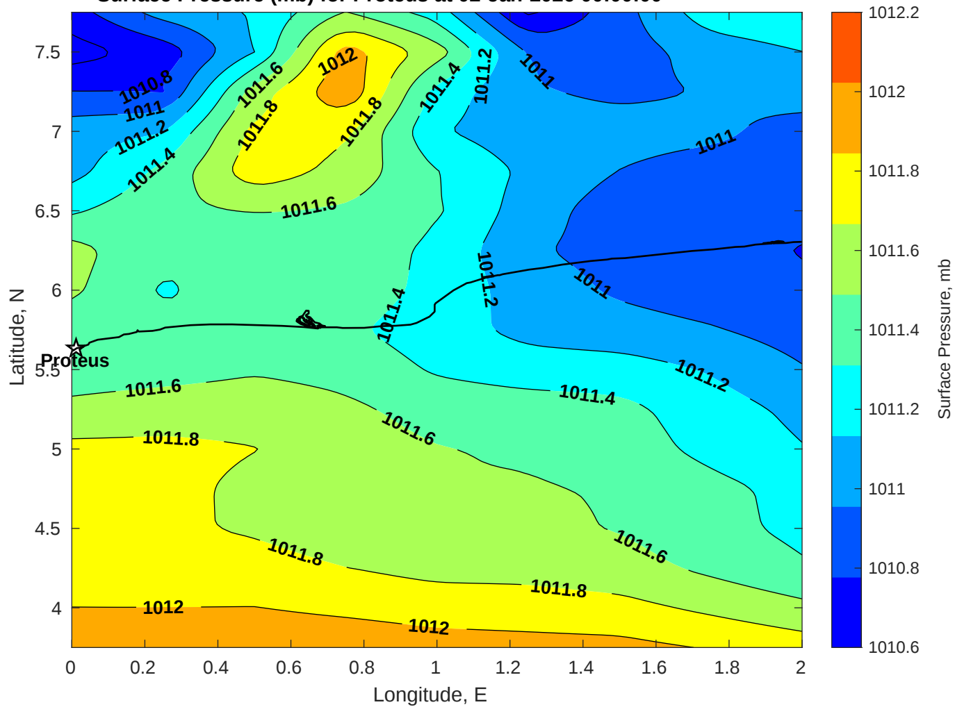
Surface Pressure (mb) for Proteus at 02-Jan-2026 00:00:00
