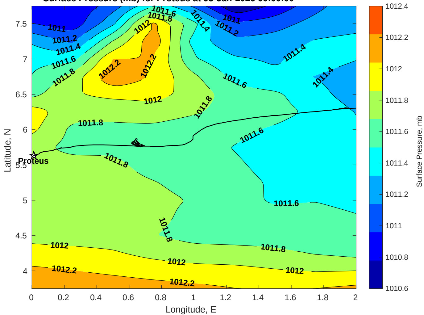
Surface Pressure (mb) for Proteus at 03-Jan-2026 00:00:00
