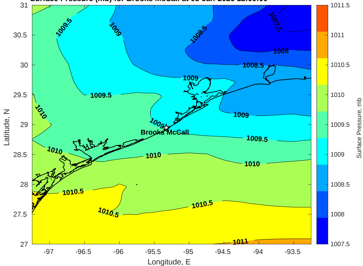
Surface Pressure (mb) for Brooks McCall at 03-Jan-2026 12:00:00
