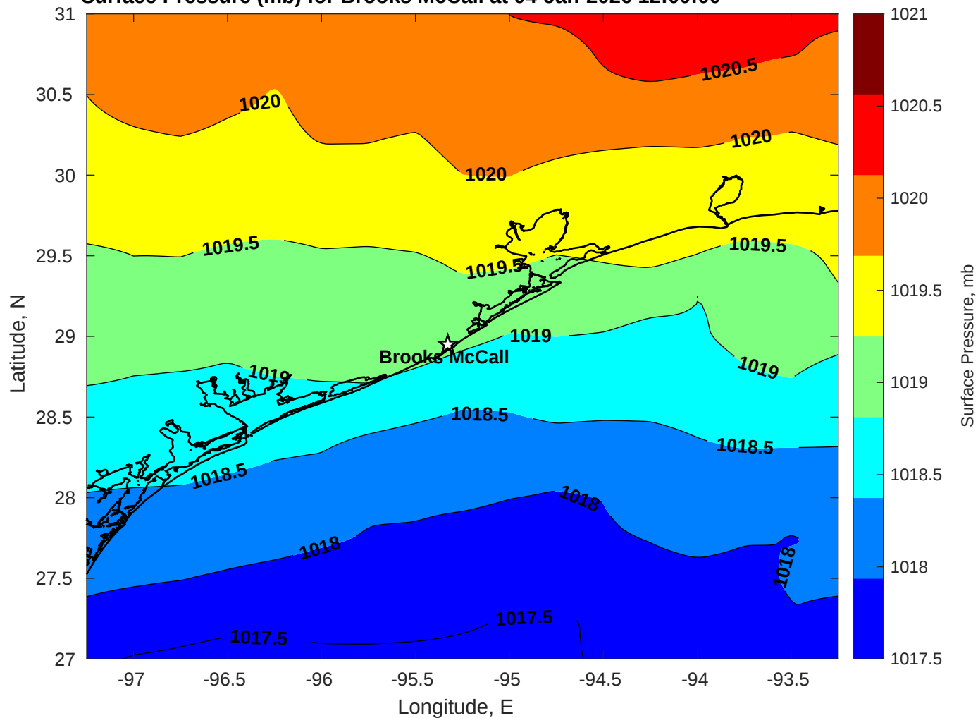
Surface Pressure (mb) for Brooks McCall at 04-Jan-2026 12:00:00
