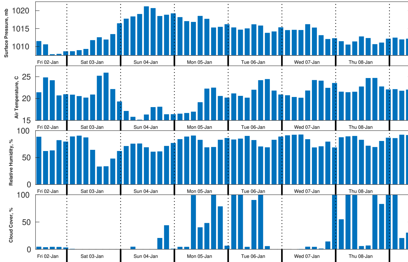
Met Forecast for Brooks McCall from 02-Jan-2026 12:00:00 to 09-Jan-2026 12:00:00
