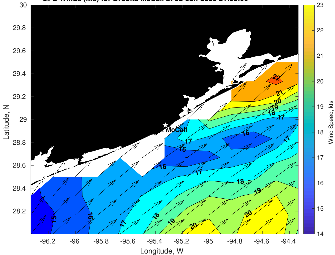
GFS Winds (kts) for Brooks McCall at 02-Jan-2026 21:00:00
