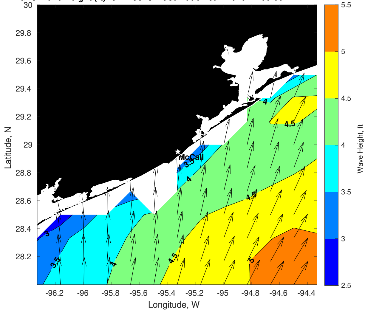
GFS Wave Height (ft) for Brooks McCall at 02-Jan-2026 21:00:00
