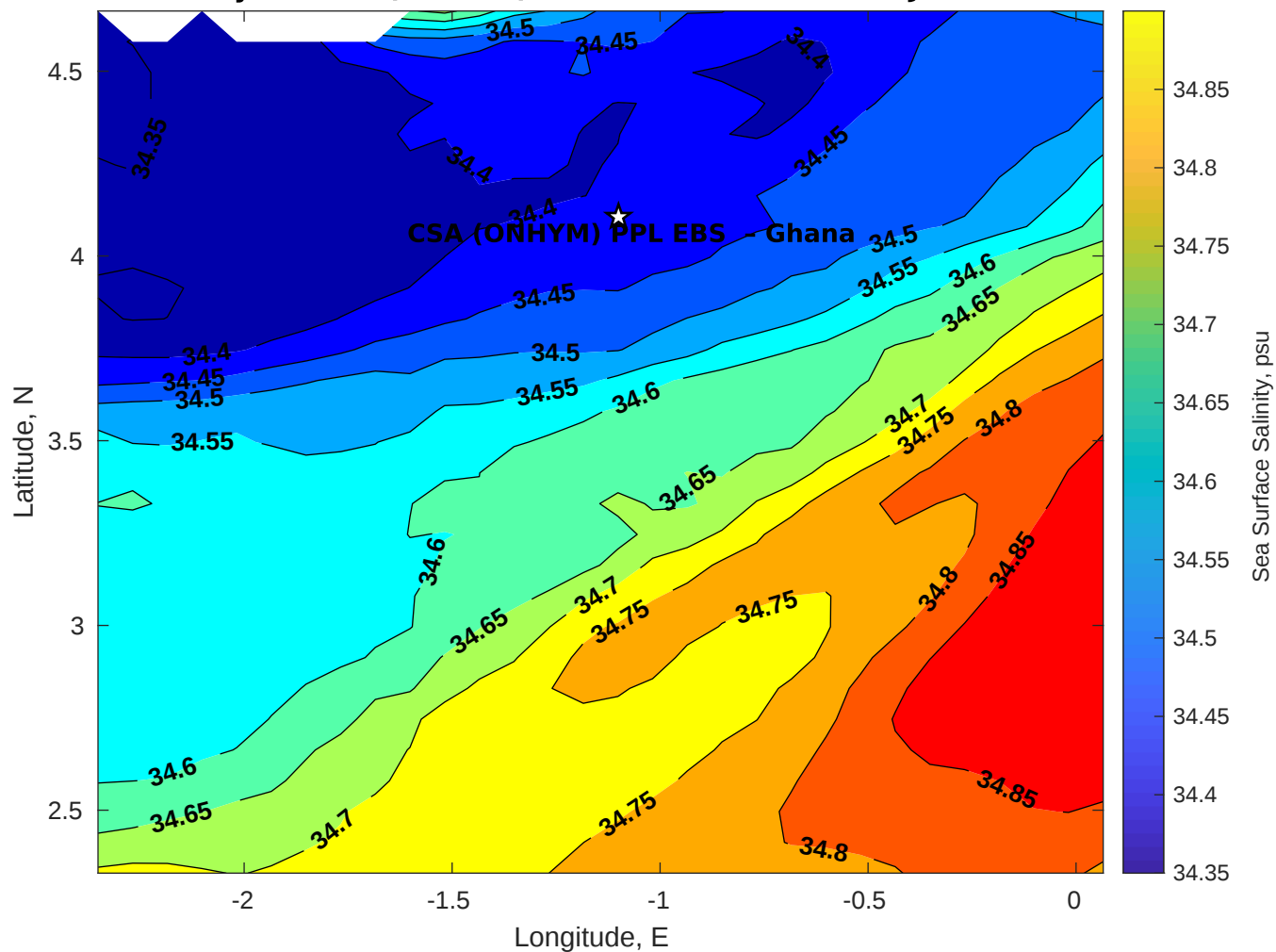
Surface Salinity for CSA (ONHYM) PPL EBS - Ghana at 02-Jan-2026 00:00:00
