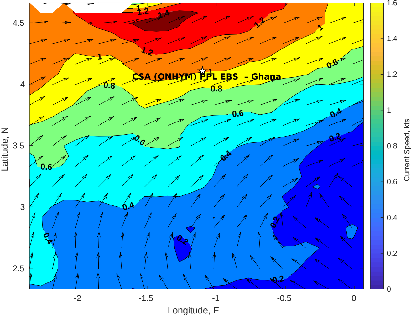
Surface Currents for CSA (ONHYM) PPL EBS - Ghana at 02-Jan-2026 00:00:00
