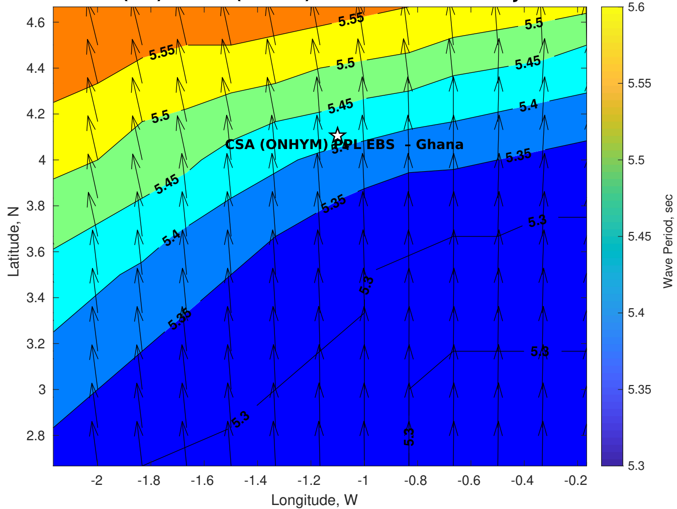
GFS Wave Period (sec) for CSA (ONHYM) PPL EBS - Ghana at 02-Jan-2026 21:00:00
