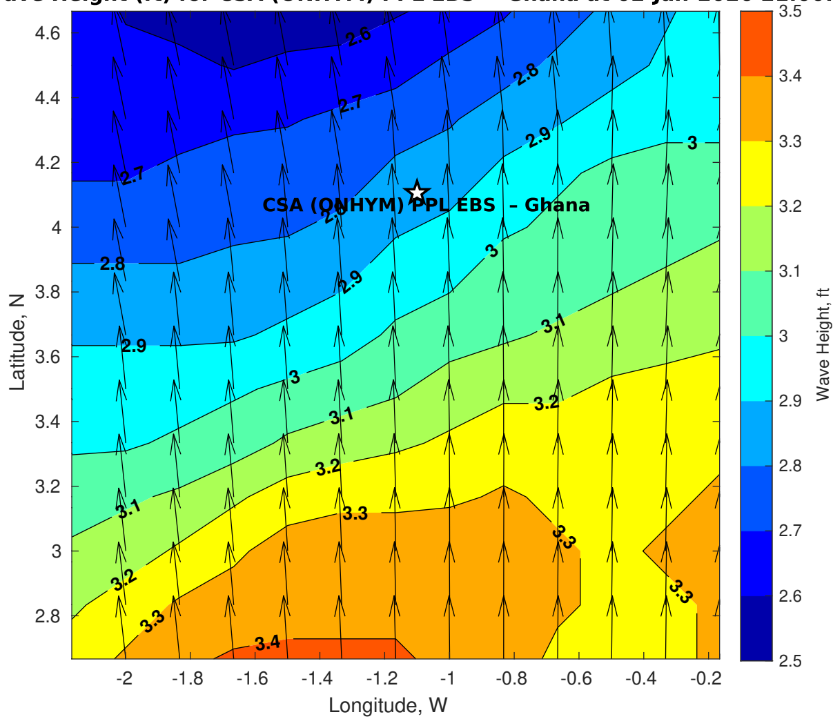
GFS Wave Height (ft) for CSA (ONHYM) PPL EBS - Ghana at 02-Jan-2026 21:00:00
