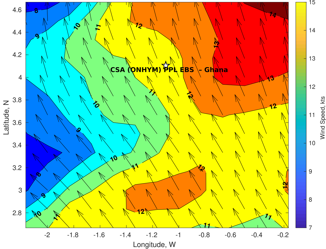
GFS Winds (kts) for CSA (ONHYM) PPL EBS - Ghana at 02-Jan-2026 21:00:00
