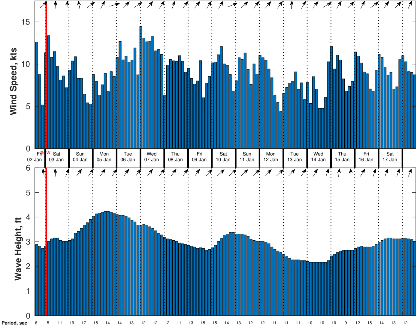
Wind & Wave Forecast for CSA (ONHYM) PPL EBS - Ghana from 02-Jan-2026 14:00:00 to 18-Jan-2026 14:00:00
