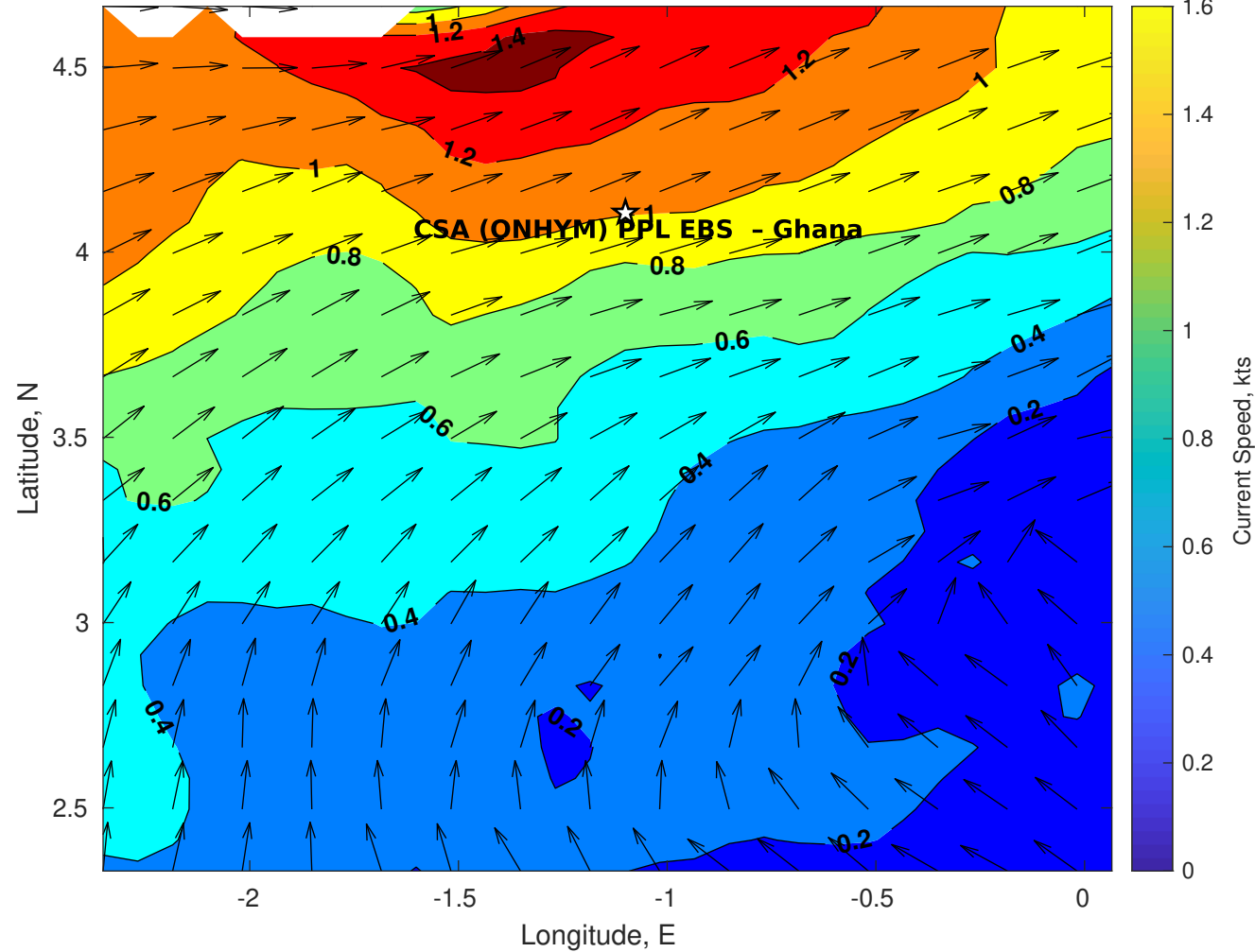
Surface Currents for CSA (ONHYM) PPL EBS - Ghana at 02-Jan-2026 00:00:00
