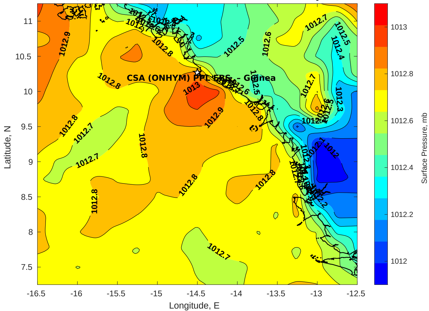
Surface Pressure (mb) for CSA (ONHYM) PPL EBS - Guinea at 02-Jan-2026 12:00:00
