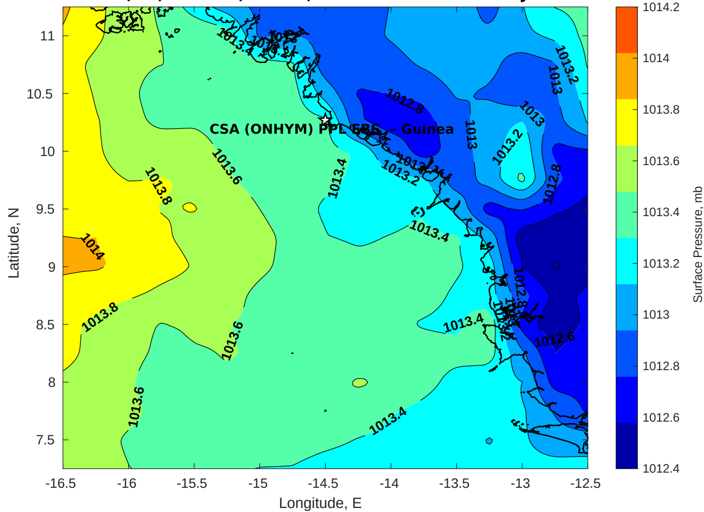
Surface Pressure (mb) for CSA (ONHYM) PPL EBS - Guinea at 03-Jan-2026 12:00:00
