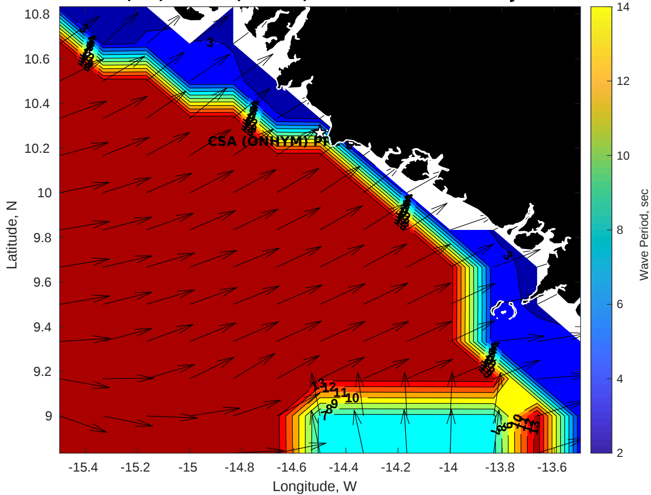
GFS Wave Period (sec) for CSA (ONHYM) PPL EBS - Guinea at 02-Jan-2026 21:00:00
