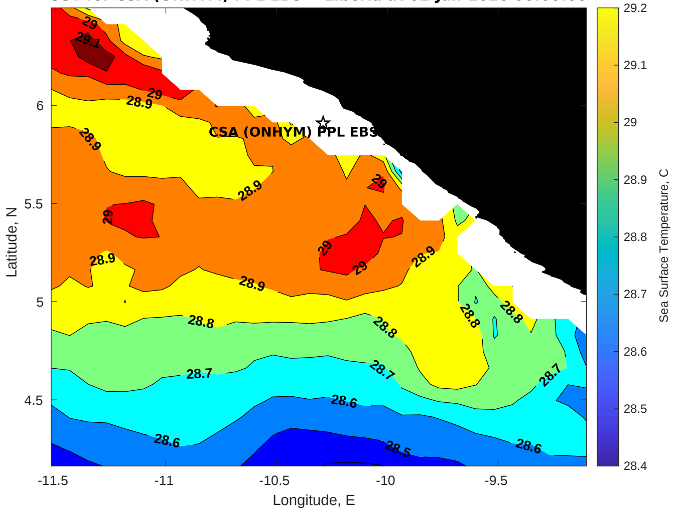
SST for CSA (ONHYM) PPL EBS - Liberia at 02-Jan-2026 00:00:00
