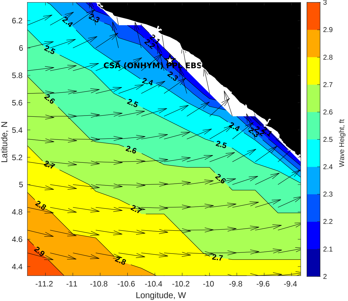
GFS Wave Height (ft) for CSA (ONHYM) PPL EBS - Liberia at 02-Jan-2026 21:00:00
