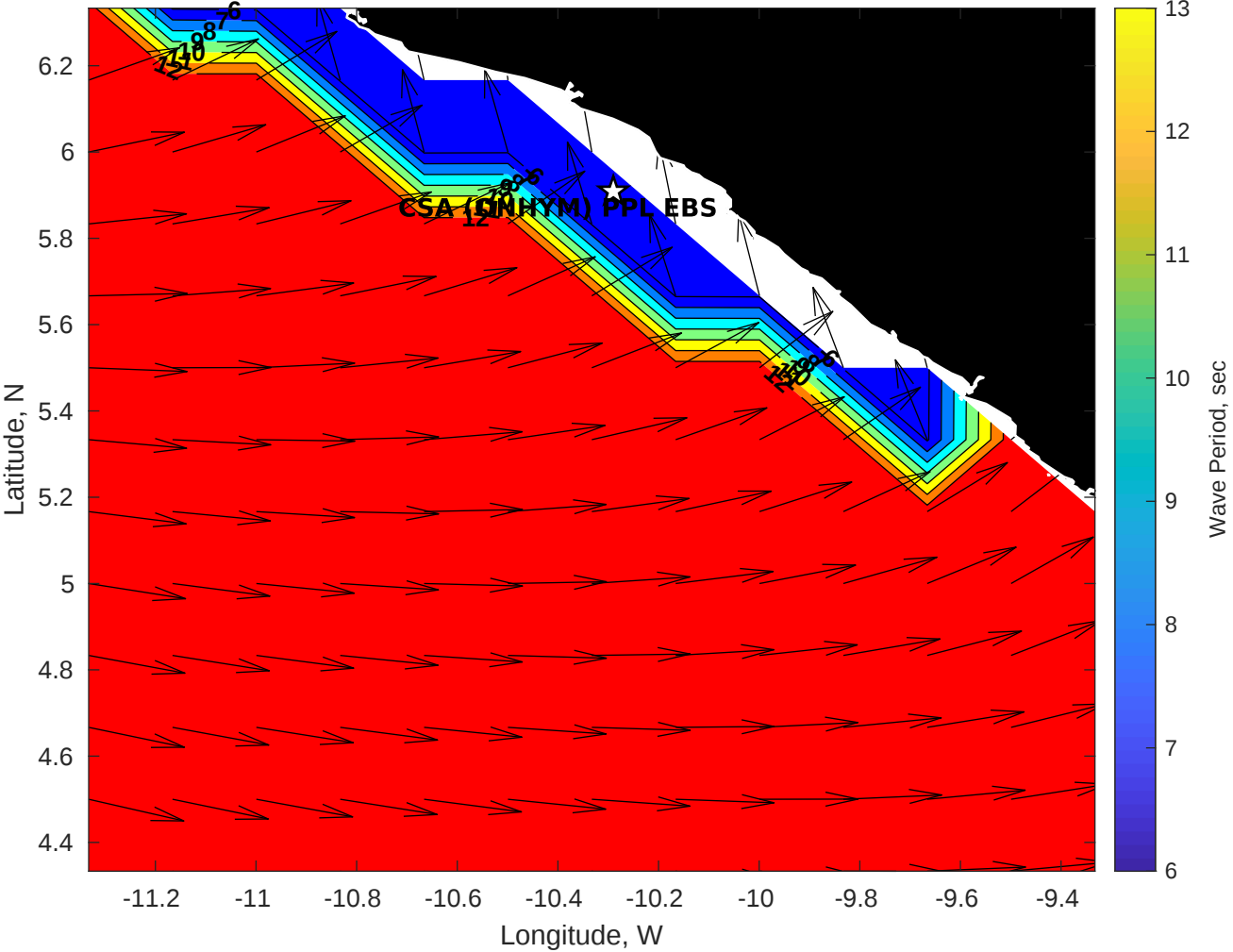
GFS Wave Period (sec) for CSA (ONHYM) PPL EBS - Liberia at 02-Jan-2026 21:00:00
