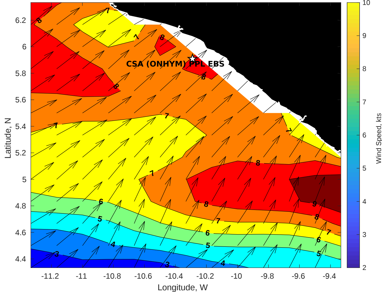
GFS Winds (kts) for CSA (ONHYM) PPL EBS - Liberia at 02-Jan-2026 21:00:00
