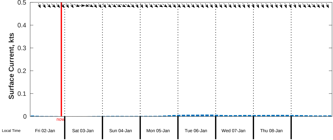
Surface Current Forecast for CSA (ONHYM) PPL EBS - Liberia from 02-Jan-2026 00:00:00 to 10-Jan-2026 00:00:00
