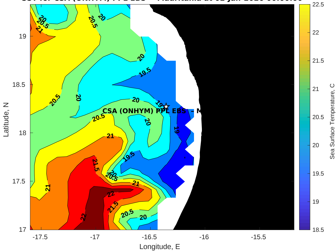
SST for CSA (ONHYM) PPL EBS - Mauritania at 02-Jan-2026 00:00:00
