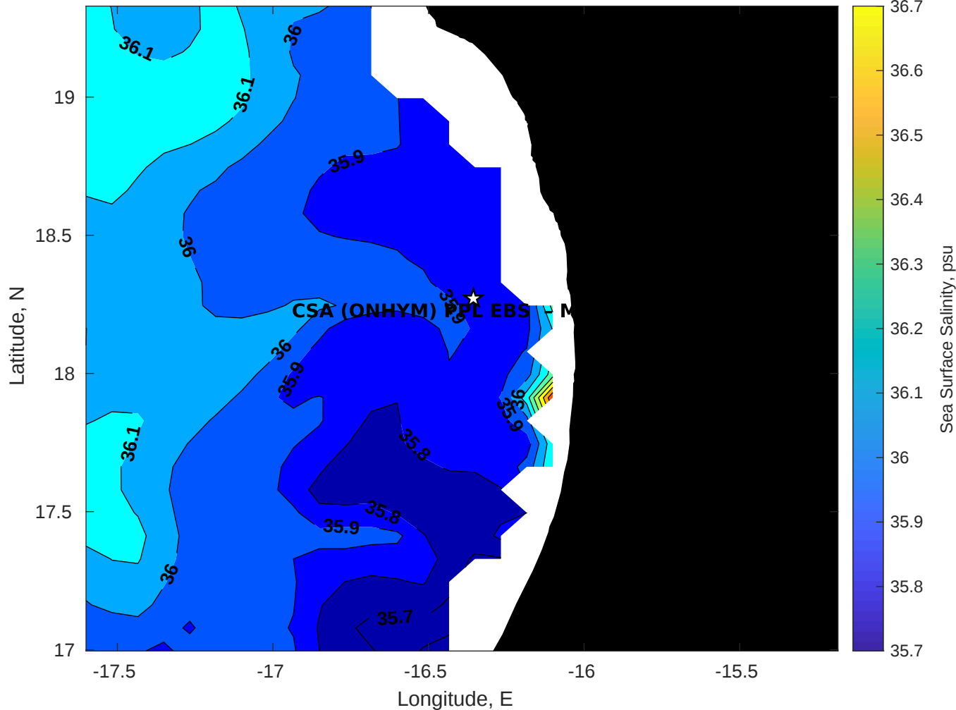
Surface Salinity for CSA (ONHYM) PPL EBS - Mauritania at 02-Jan-2026 00:00:00
