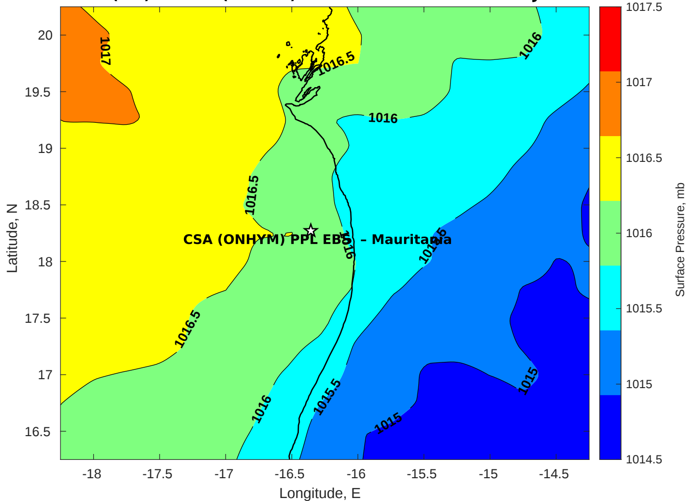
Surface Pressure (mb) for CSA (ONHYM) PPL EBS - Mauritania at 04-Jan-2026 12:00:00
