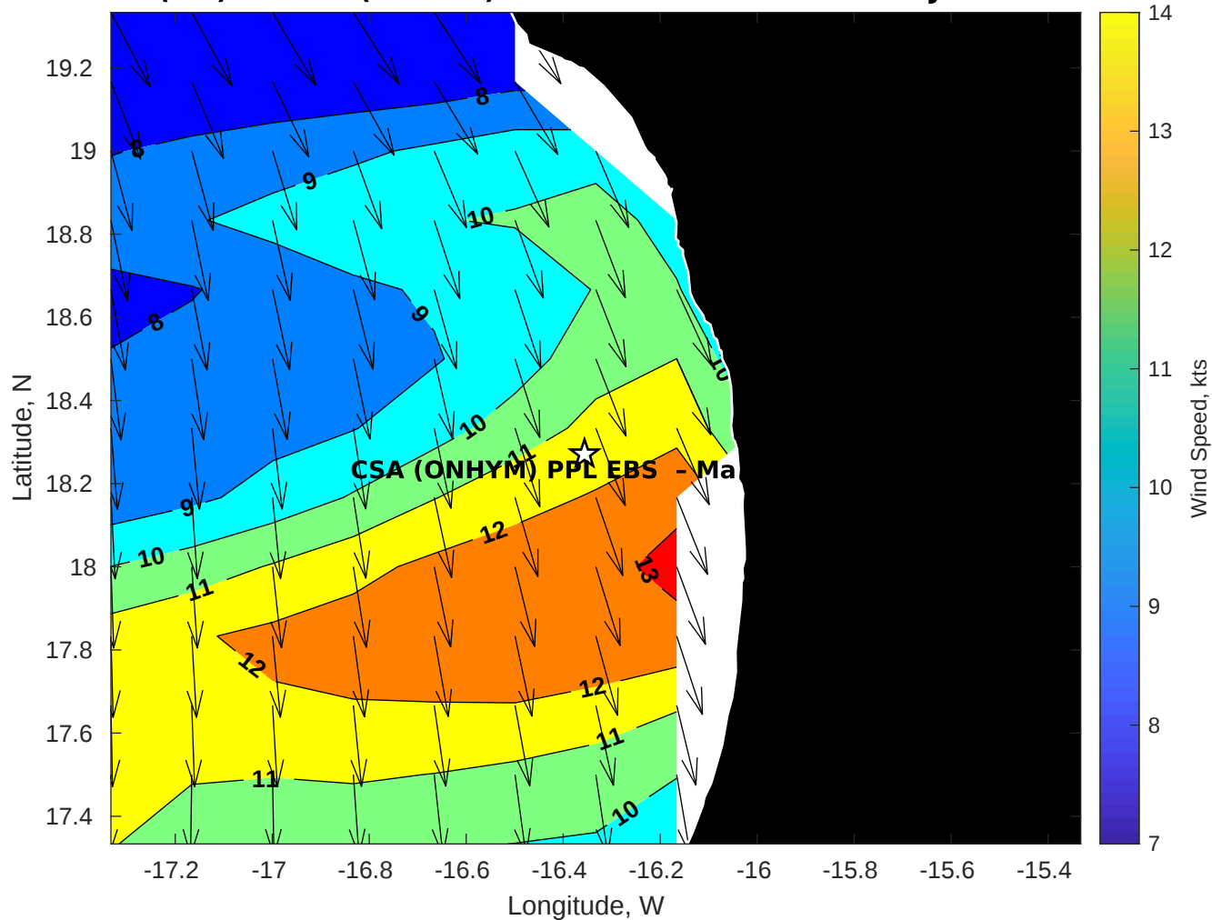
GFS Winds (kts) for CSA (ONHYM) PPL EBS - Mauritania at 02-Jan-2026 21:00:00
