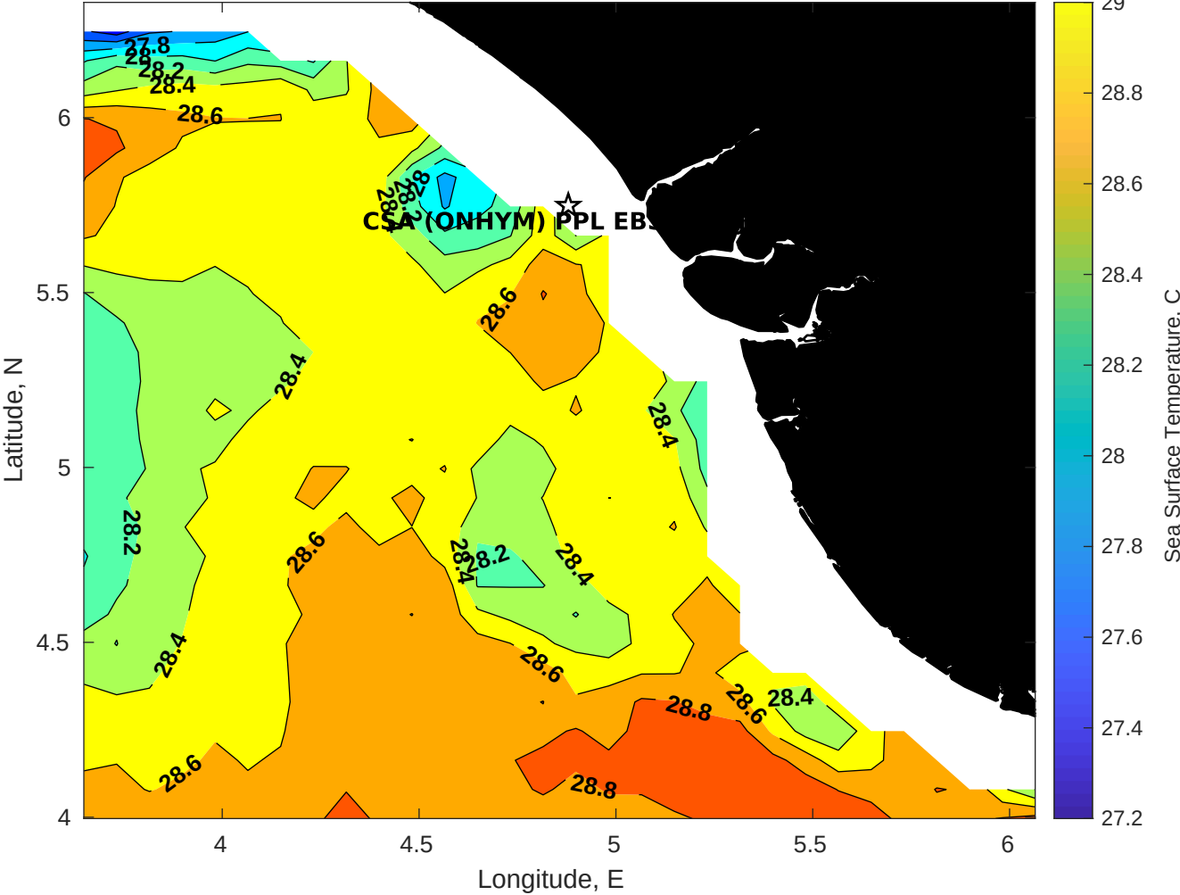
SST for CSA (ONHYM) PPL EBS - Nigeria at 02-Jan-2026 00:00:00
