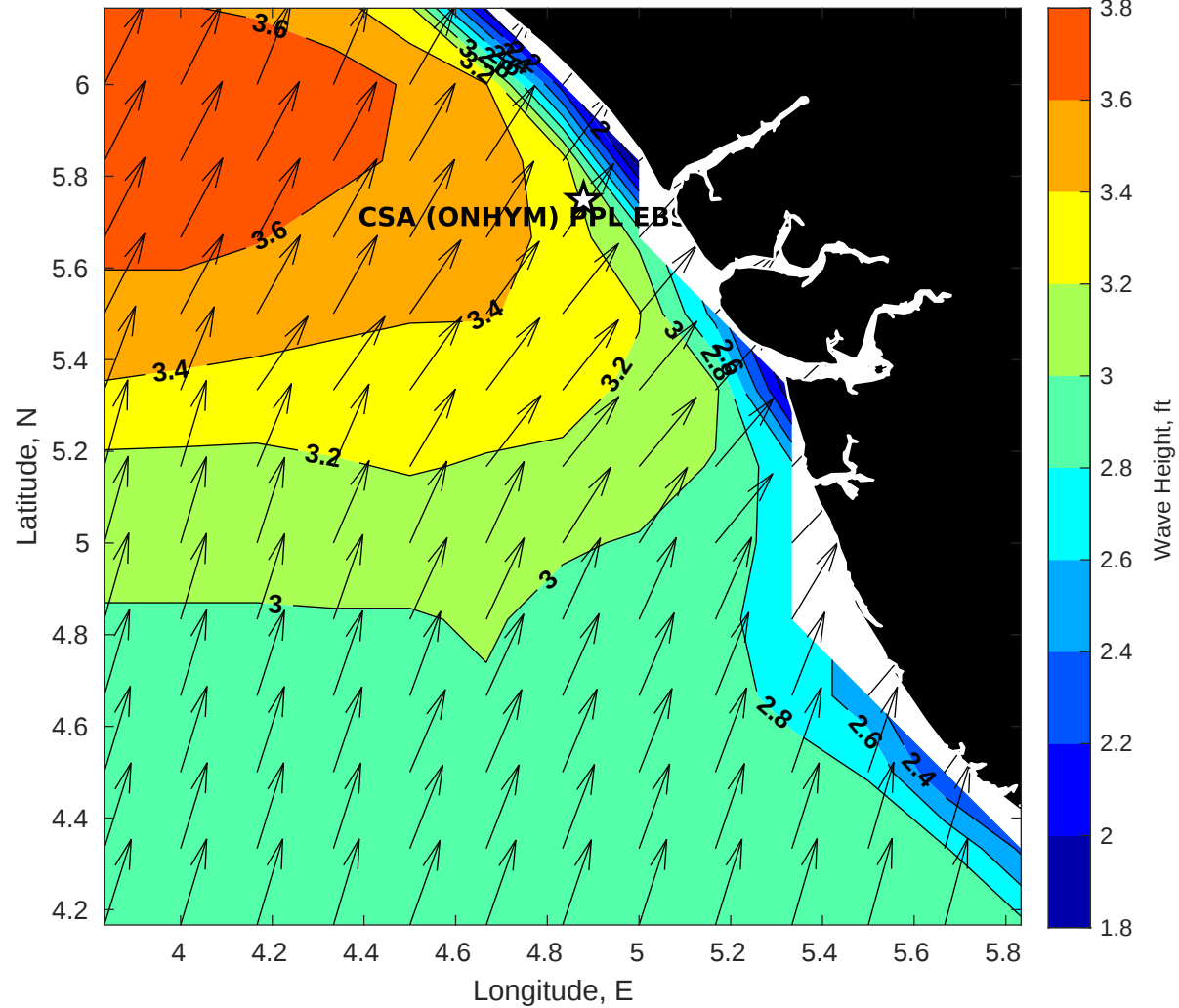
GFS Wave Height (ft) for CSA (ONHYM) PPL EBS - Nigeria at 02-Jan-2026 21:00:00
