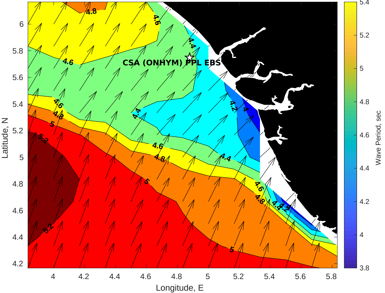
GFS Wave Period (sec) for CSA (ONHYM) PPL EBS - Nigeria at 02-Jan-2026 21:00:00
