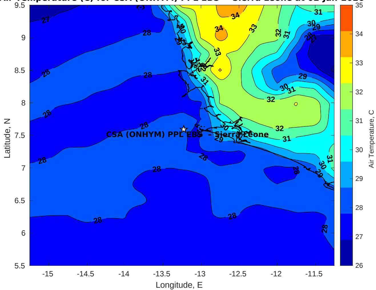
Air Temperature (C) for CSA (ONHYM) PPL EBS - Sierra Leone at 02-Jan-2026
