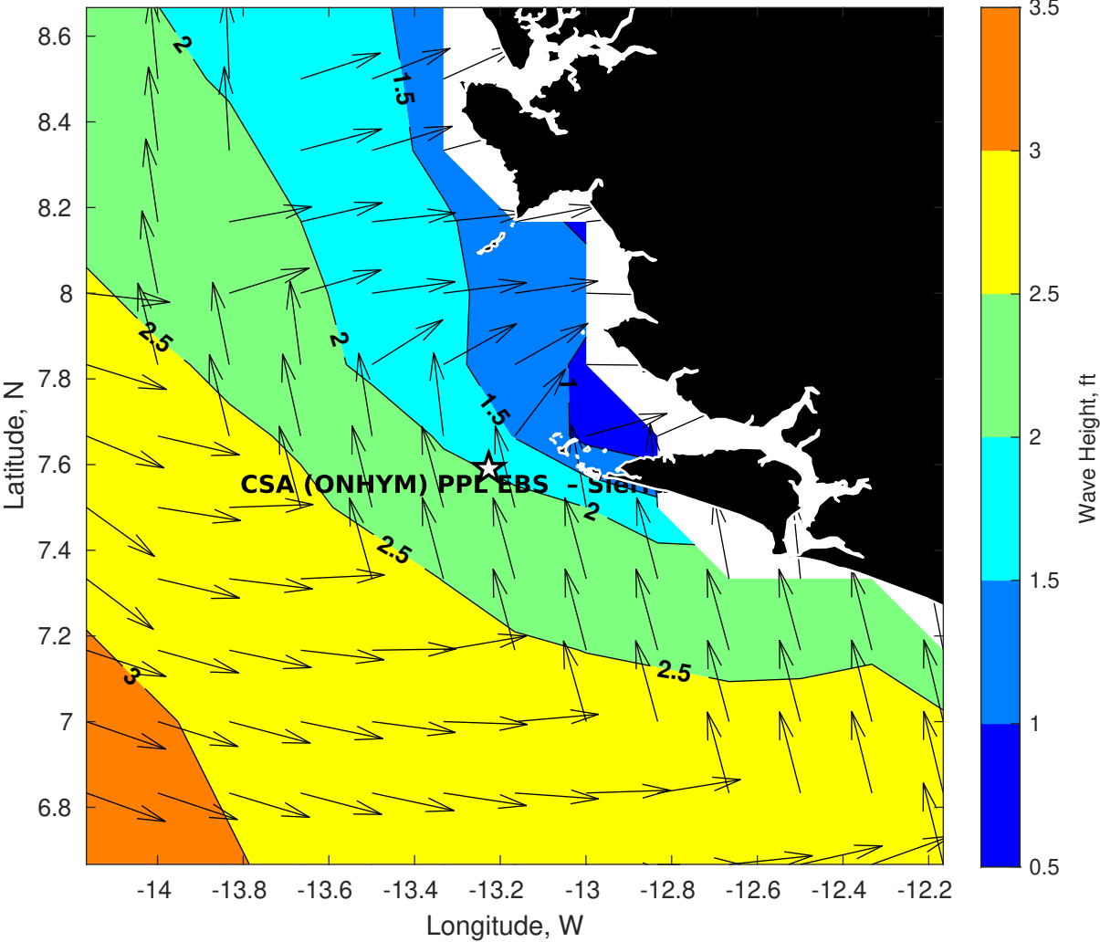
GFS Wave Height (ft) for CSA (ONHYM) PPL EBS - Sierra Leone at 02-Jan-2026 21:00:00
