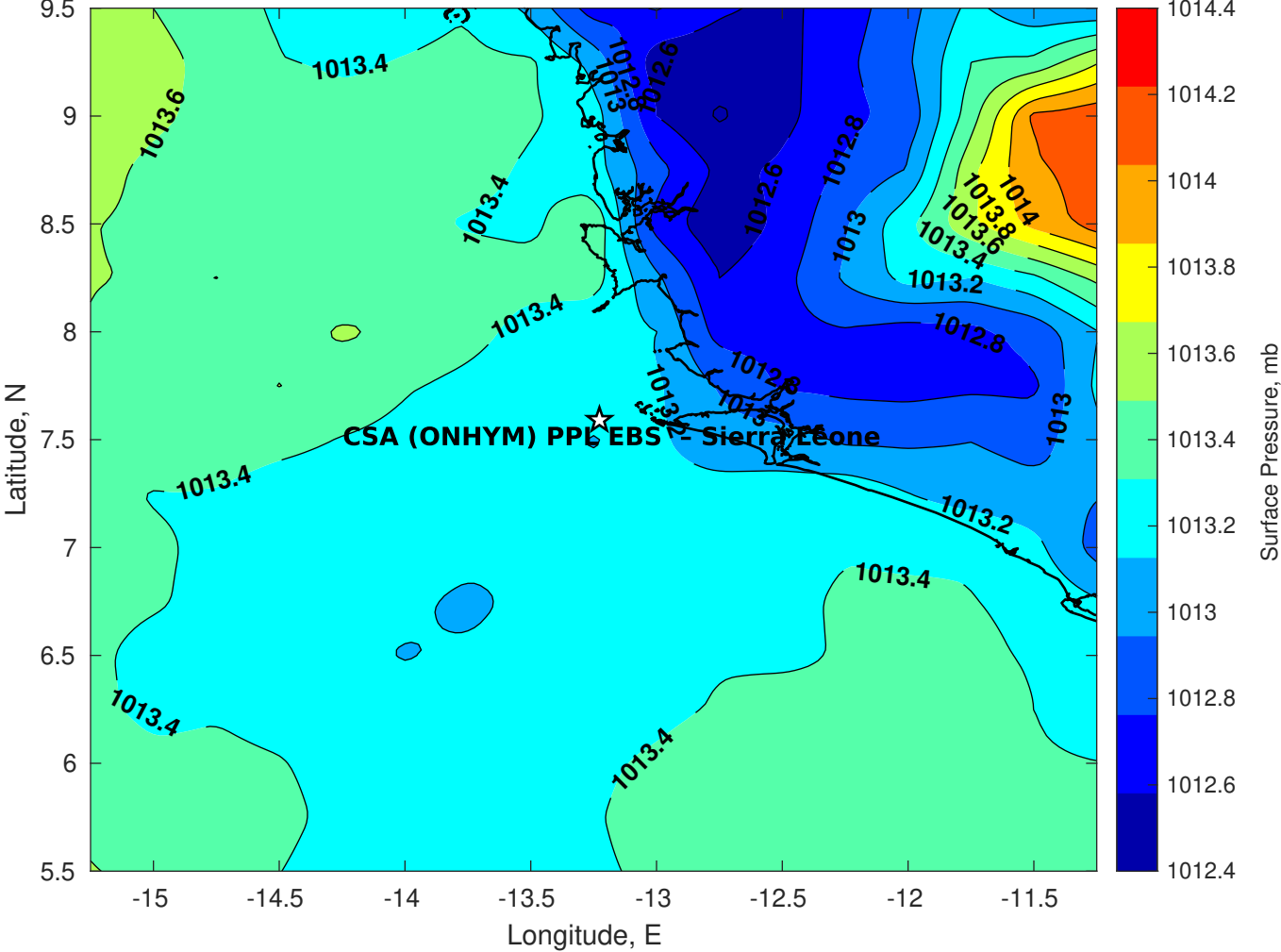
Surface Pressure (mb) for CSA (ONHYM) PPL EBS - Sierra Leone at 03-Jan-2026 12:00:00
