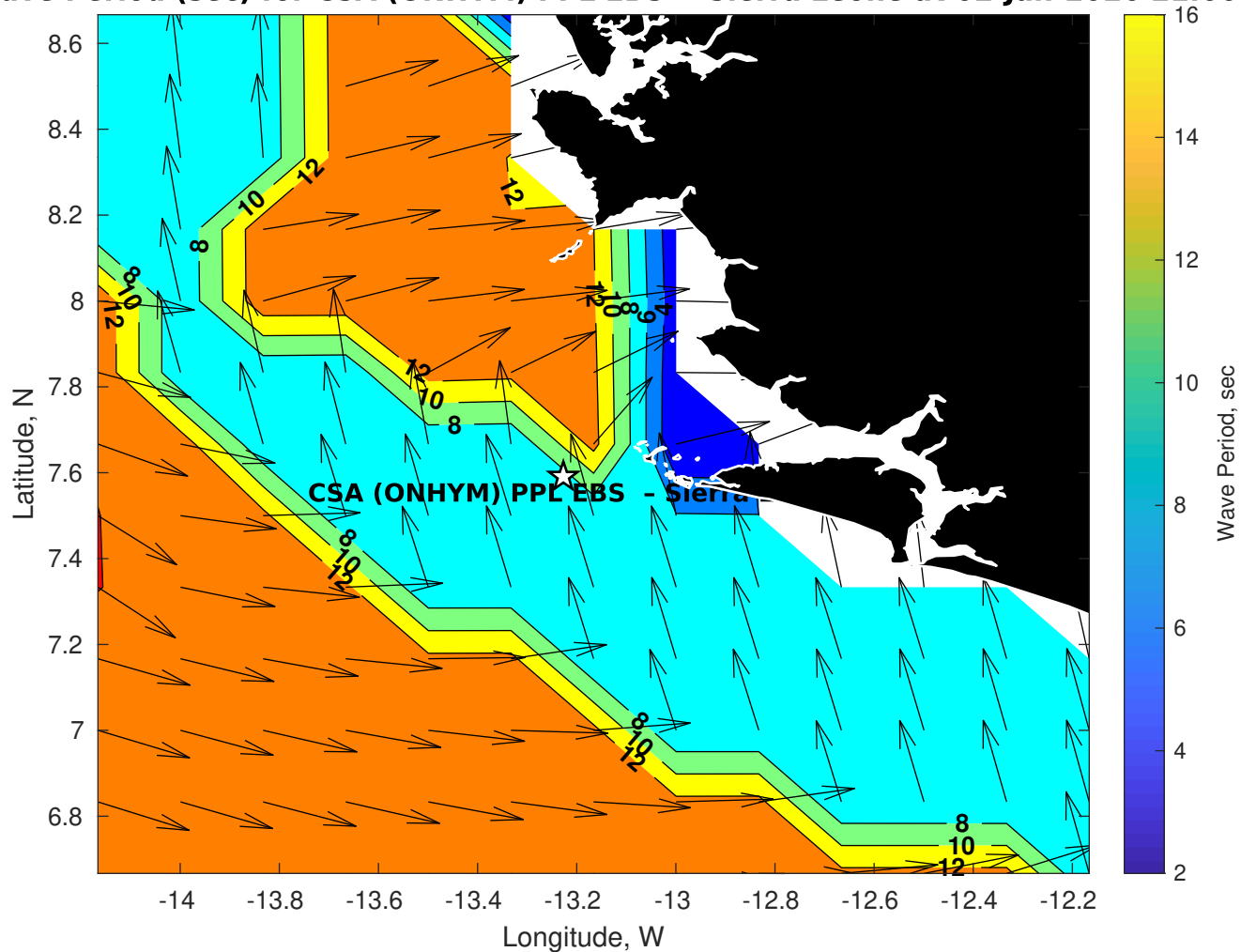
GFS Wave Period (sec) for CSA (ONHYM) PPL EBS - Sierra Leone at 02-Jan-2026 21:00:00
