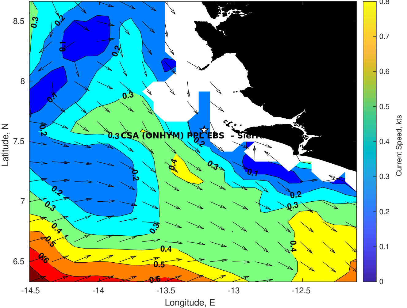
Surface Currents for CSA (ONHYM) PPL EBS - Sierra Leone at 02-Jan-2026 00:00:00
