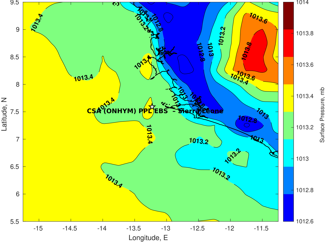
Surface Pressure (mb) for CSA (ONHYM) PPL EBS - Sierra Leone at 04-Jan-2026 12:00:00
