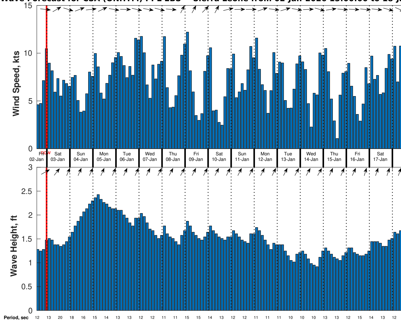
Wind & Wave Forecast for CSA (ONHYM) PPL EBS - Sierra Leone from 02-Jan-2026 13:00:00 to 18-Jan-2026 13:00:00
