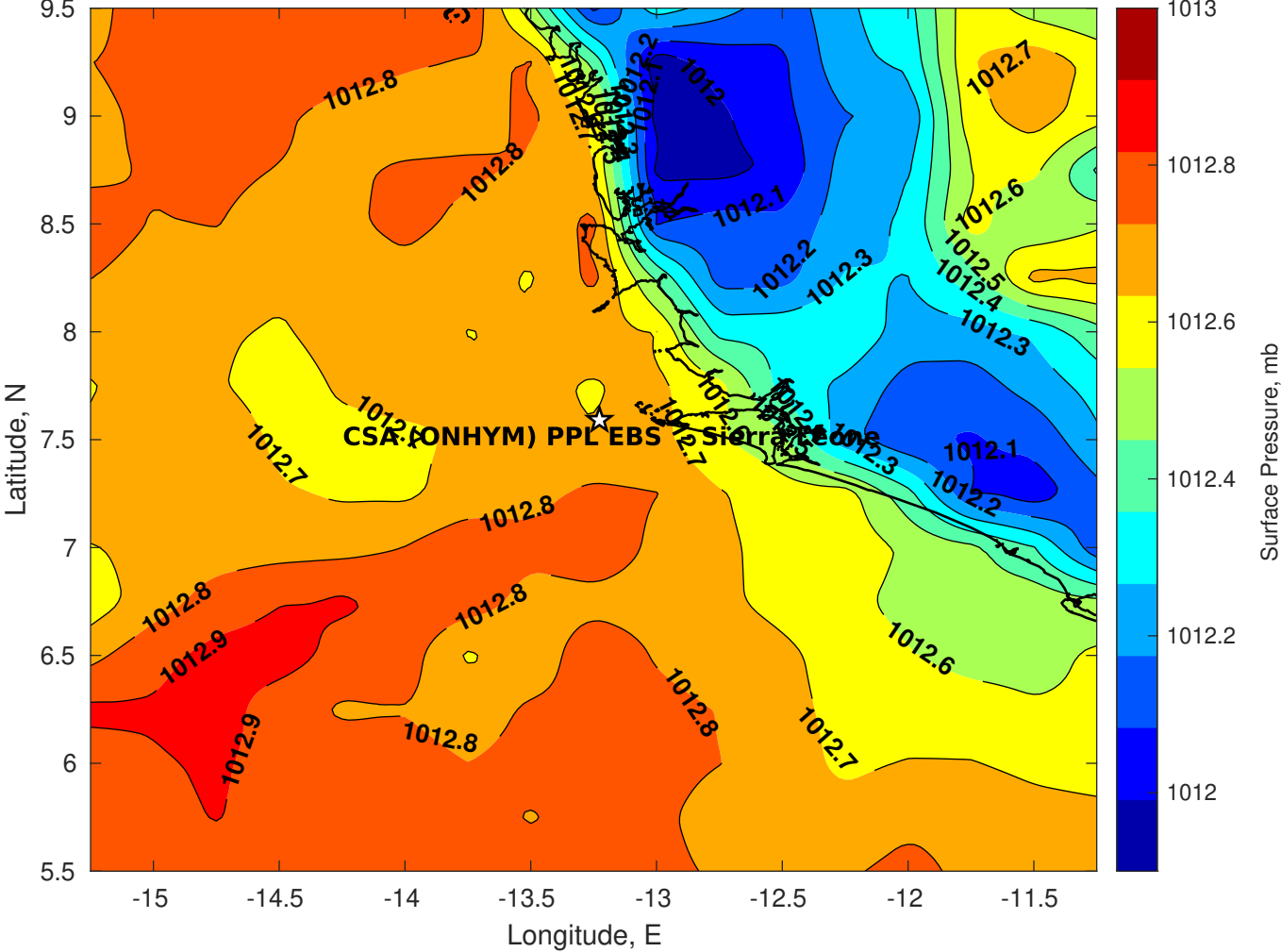
Surface Pressure (mb) for CSA (ONHYM) PPL EBS - Sierra Leone at 02-Jan-2026 12:00:00
