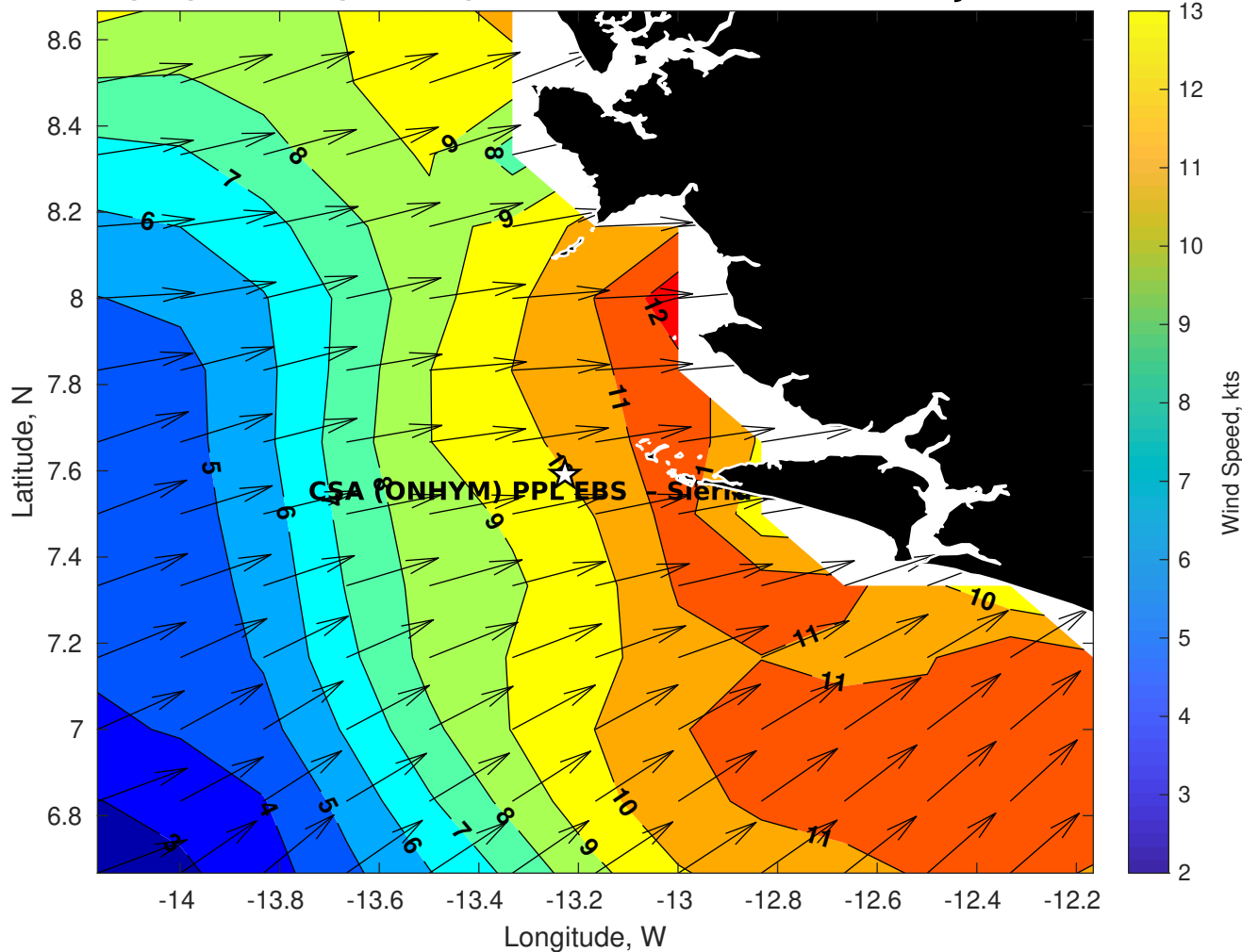
GFS Winds (kts) for CSA (ONHYM) PPL EBS - Sierra Leone at 02-Jan-2026 21:00:00
