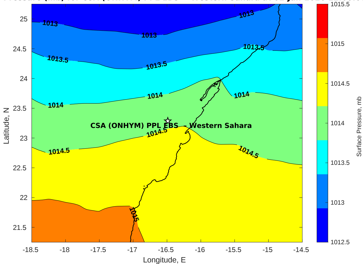
Surface Pressure (mb) for CSA (ONHYM) PPL EBS - Western Sahara at 02-Jan-2026 12:00:00
