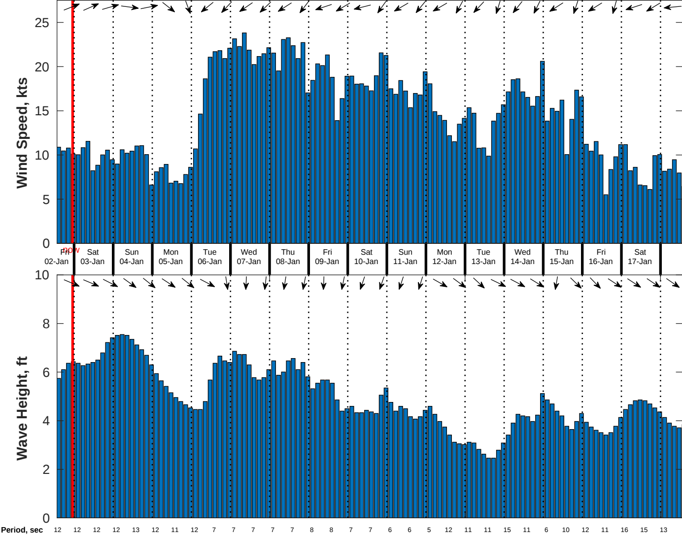
Wind & Wave Forecast for CSA (ONHYM) PPL EBS - Western Sahara from 02-Jan-2026 13:00:00 to 18-Jan-2026 13:00:00
