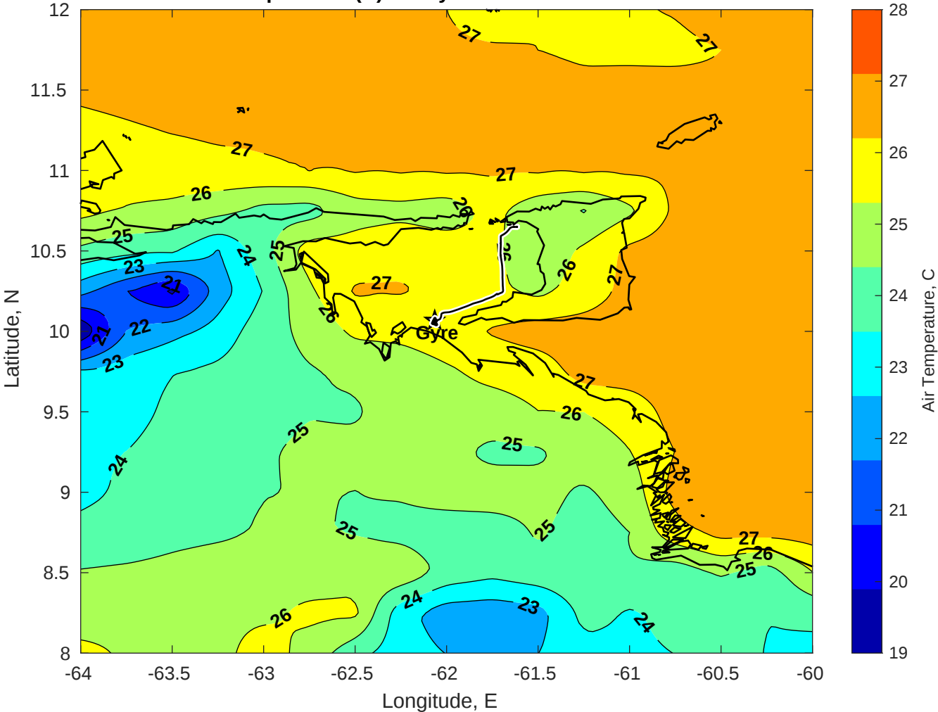
Air Temperature (C) for Gyre at 02-Jan-2026
