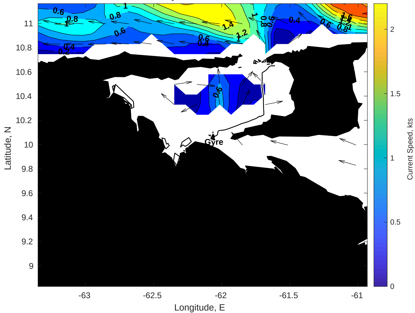
Surface Currents for Gyre at 02-Jan-2026 00:00:00
