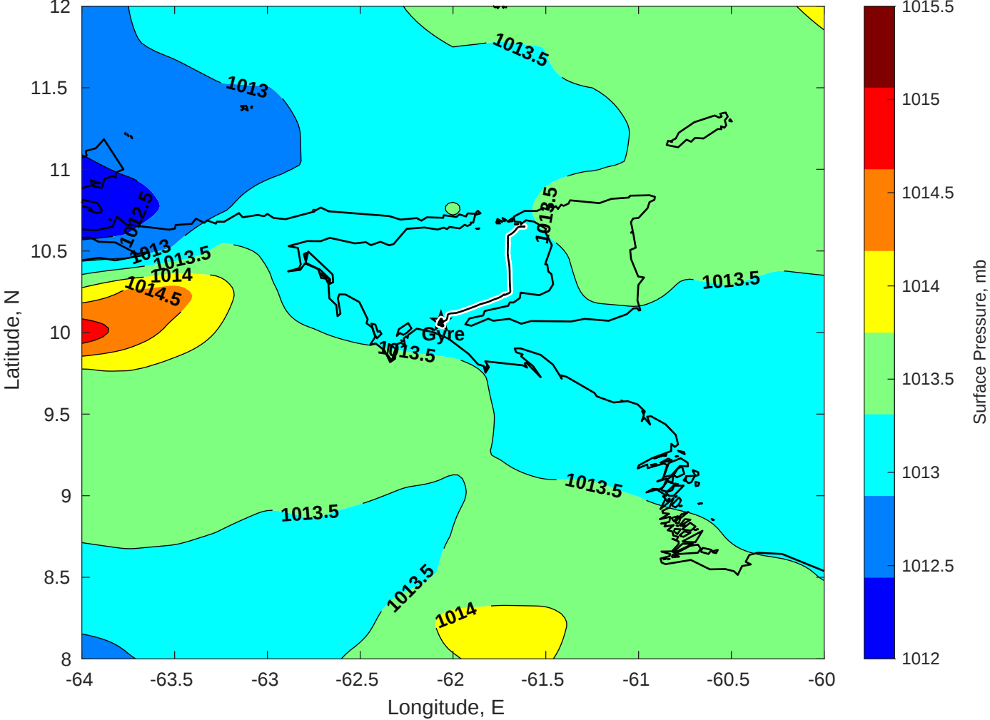
Surface Pressure (mb) for Gyre at 02-Jan-2026 12:00:00
