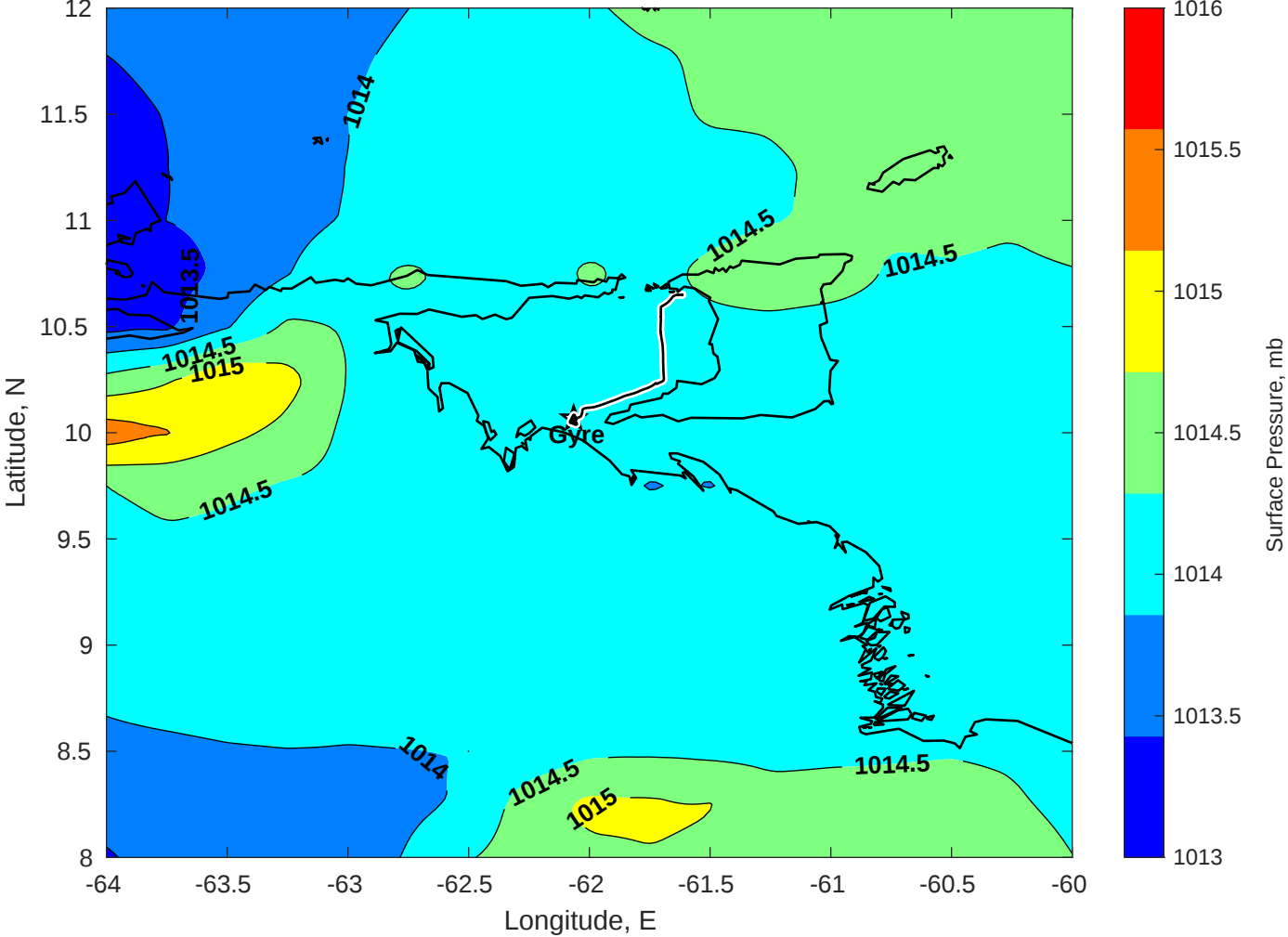
Surface Pressure (mb) for Gyre at 04-Jan-2026 12:00:00
