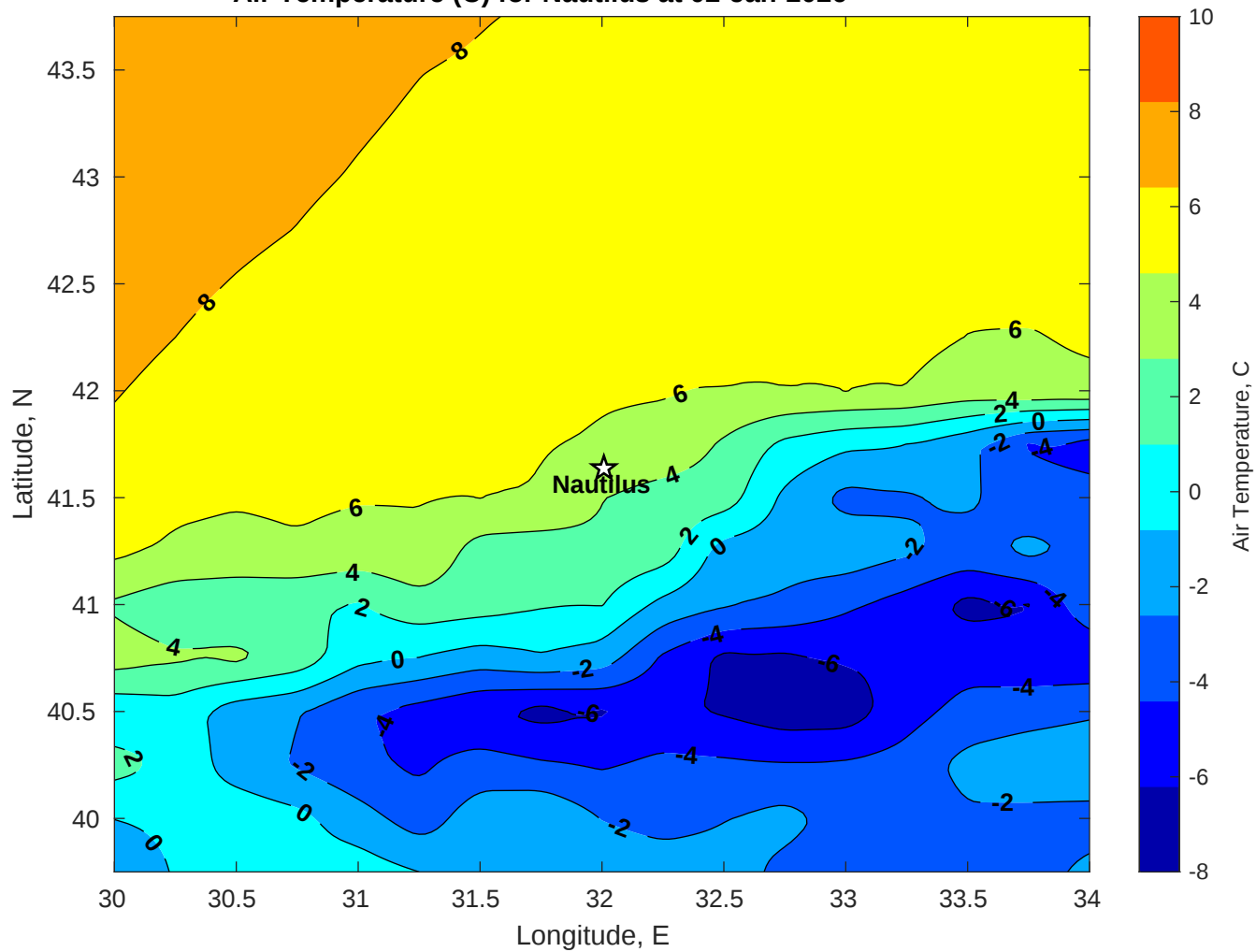
Air Temperature (C) for Nautilus at 02-Jan-2026
