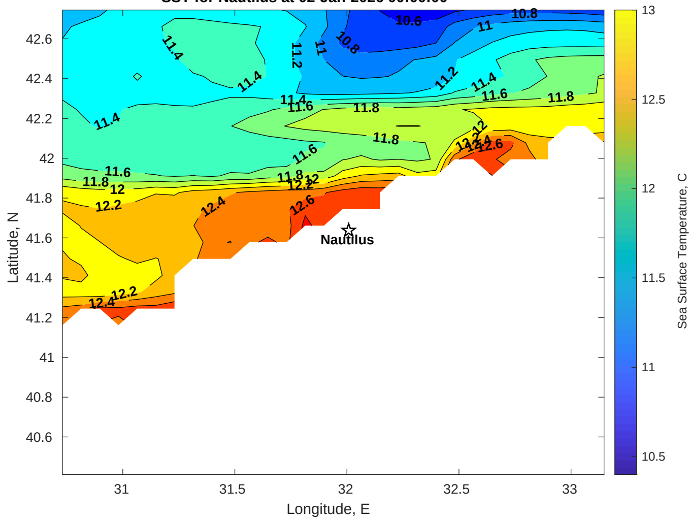
SST for Nautilus at 02-Jan-2026 00:00:00
