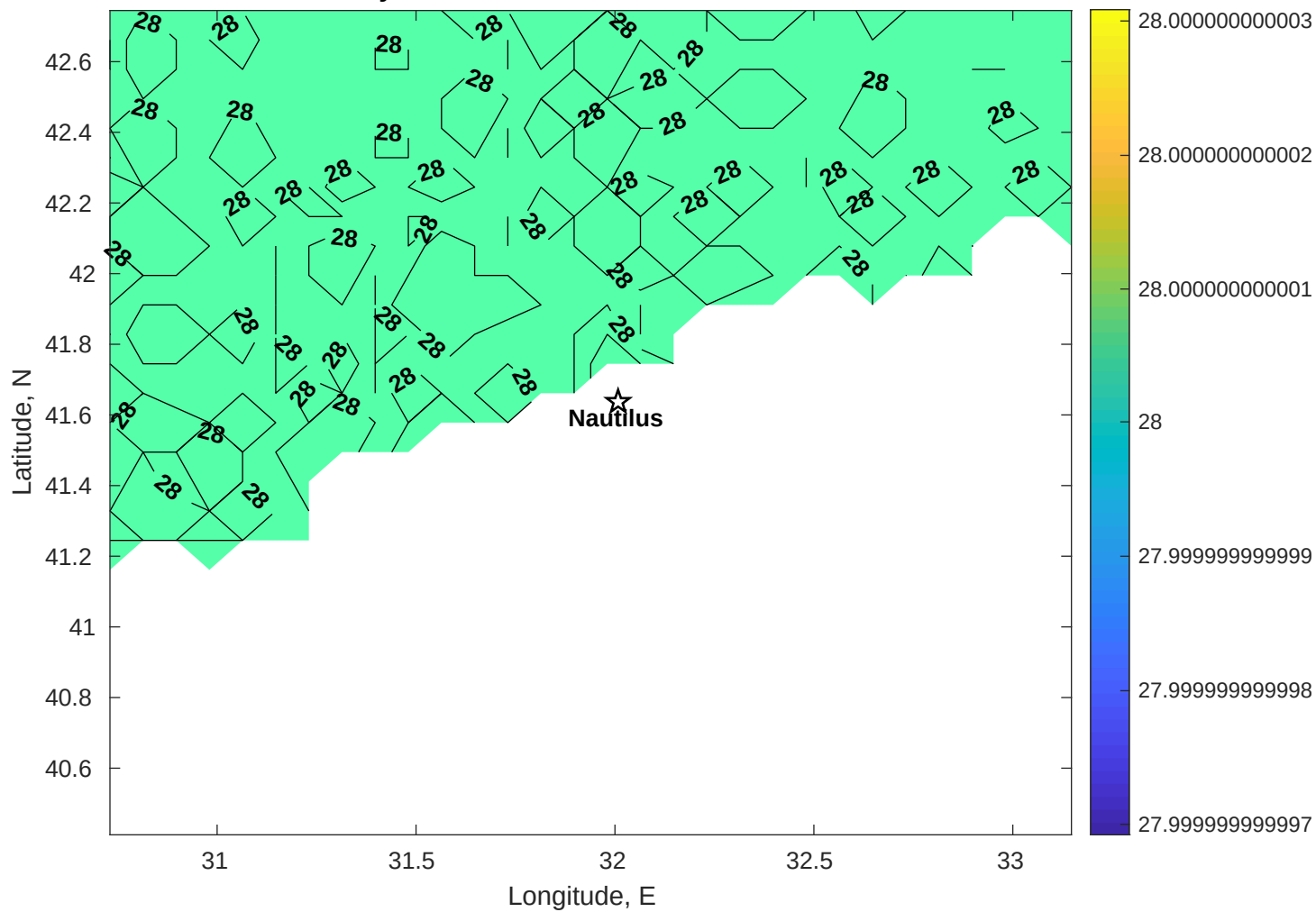
Surface Salinity for Nautilus at 02-Jan-2026 00:00:00
