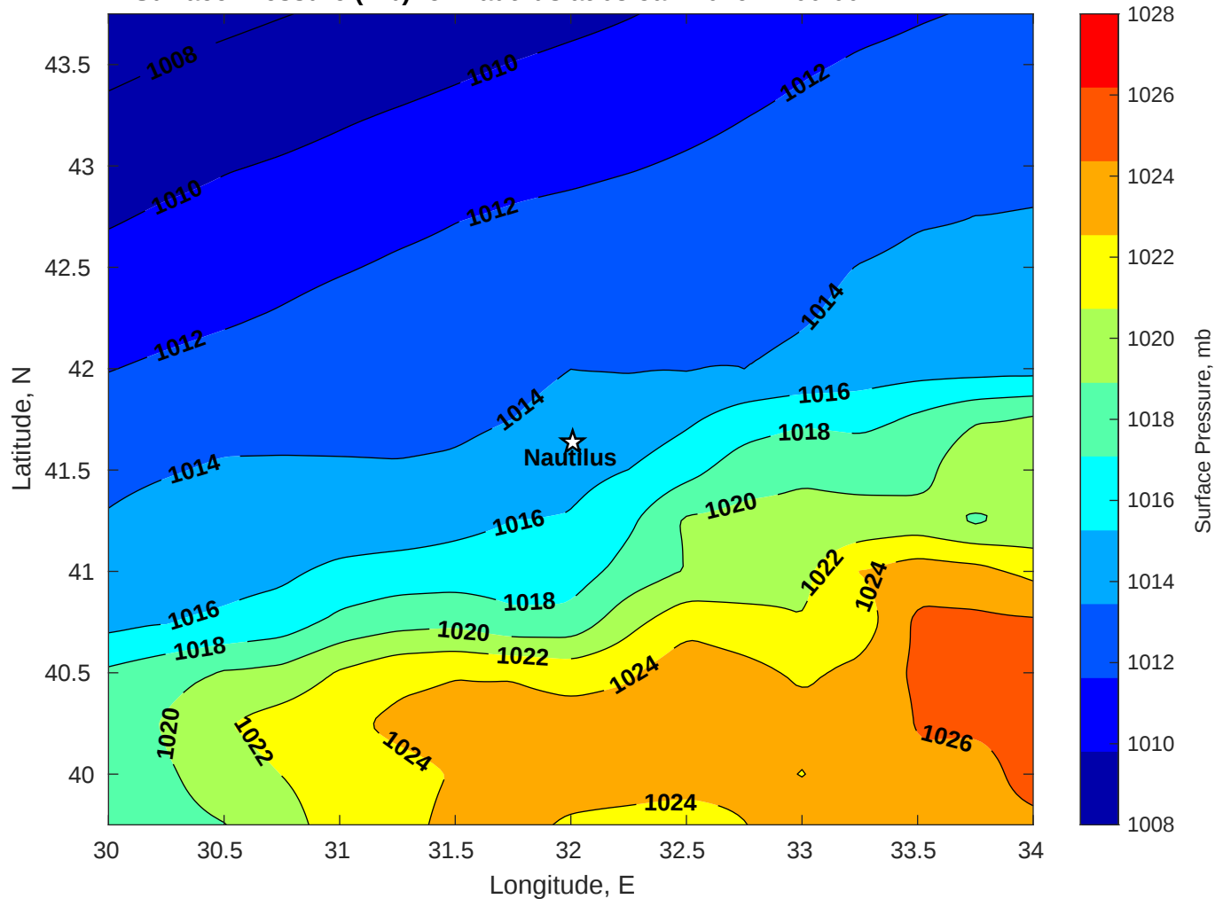
Surface Pressure (mb) for Nautilus at 03-Jan-2026 12:00:00
