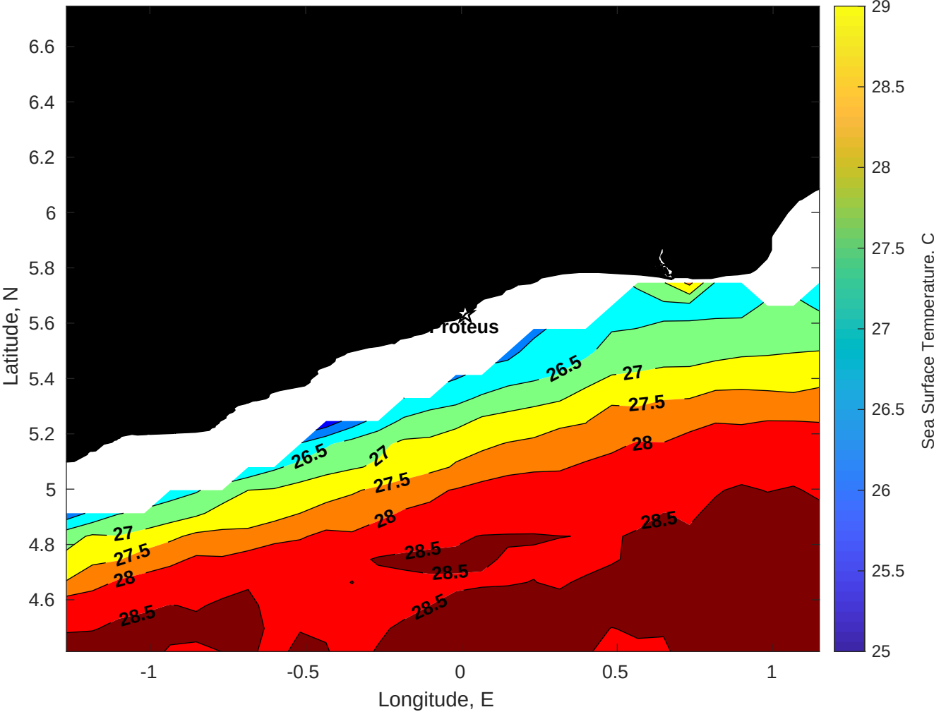
SST for Proteus at 02-Jan-2026 00:00:00
