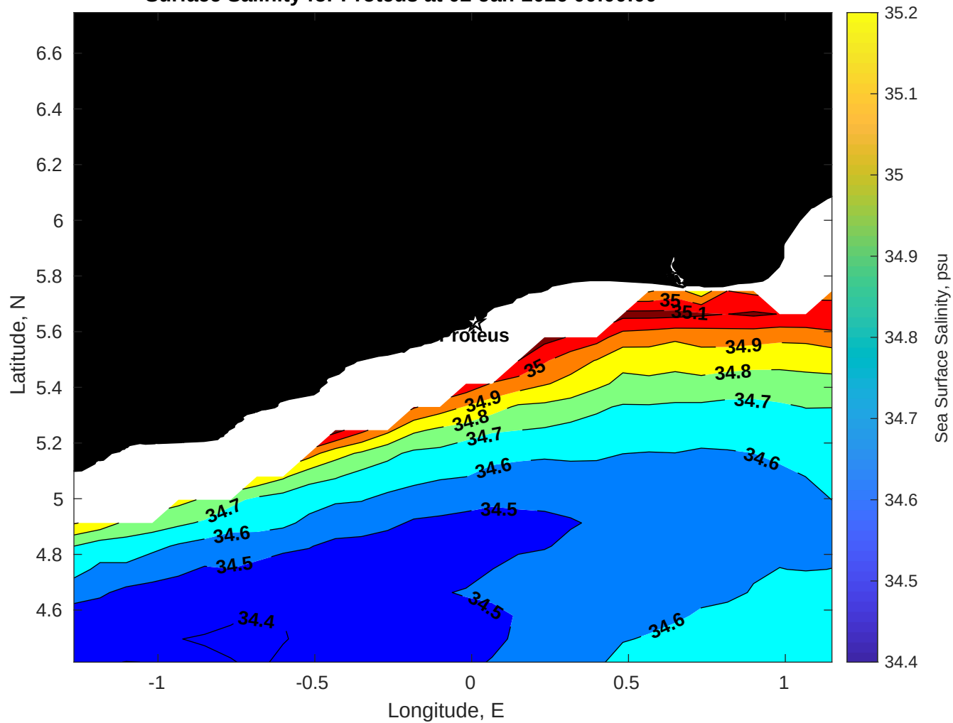
Surface Salinity for Proteus at 02-Jan-2026 00:00:00
