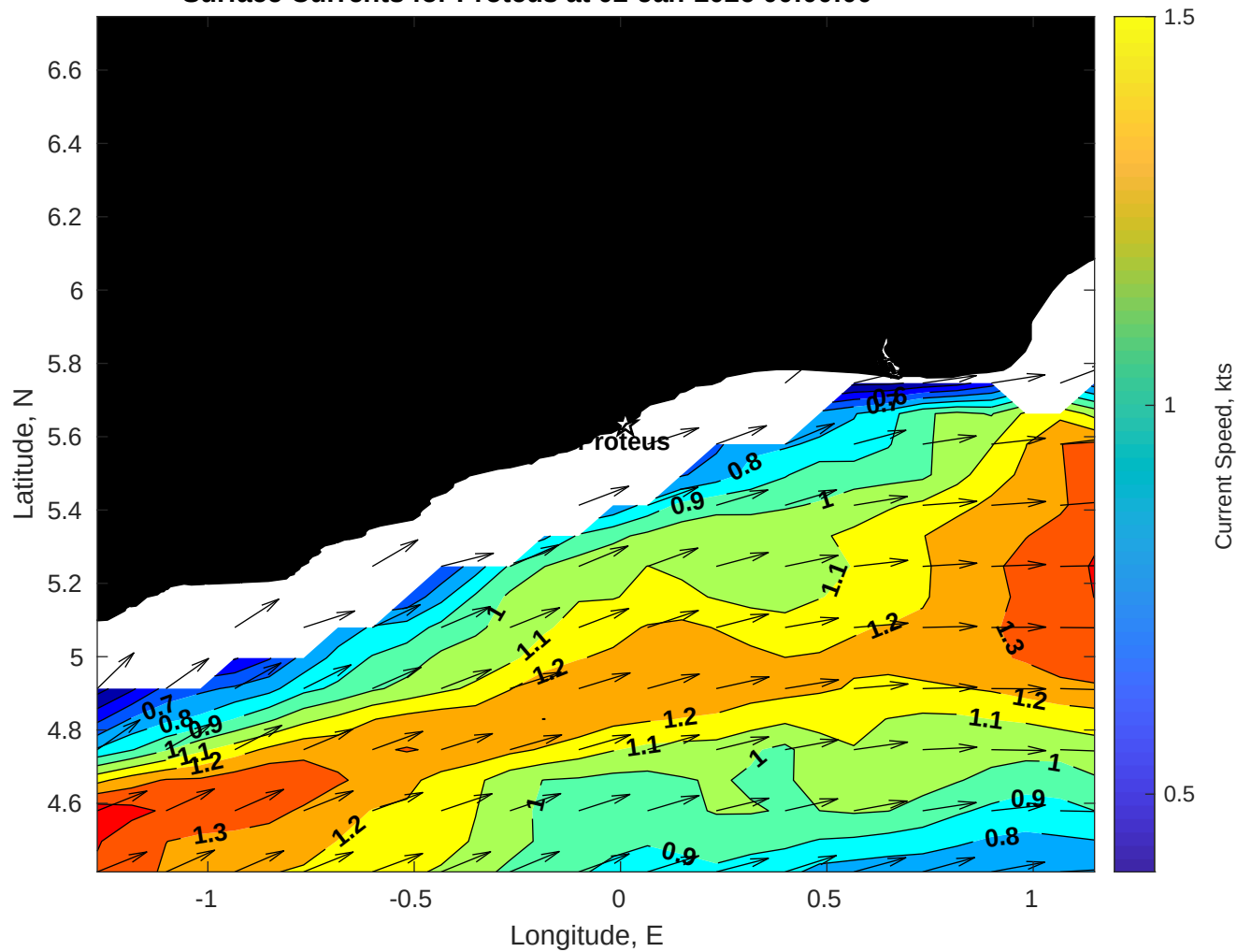
Surface Currents for Proteus at 02-Jan-2026 00:00:00
