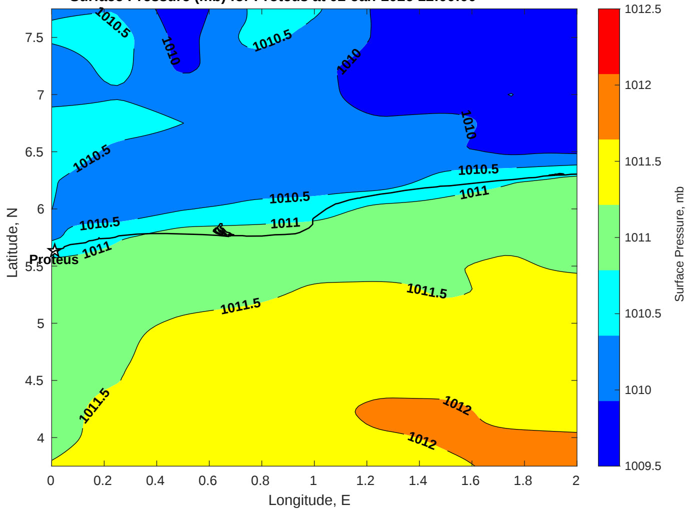
Surface Pressure (mb) for Proteus at 02-Jan-2026 12:00:00
