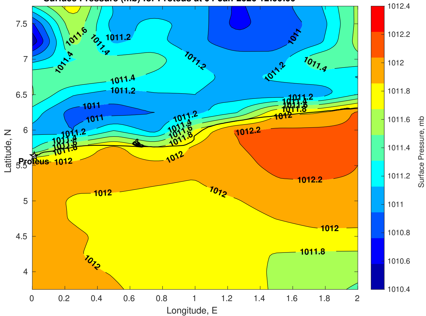
Surface Pressure (mb) for Proteus at 04-Jan-2026 12:00:00
