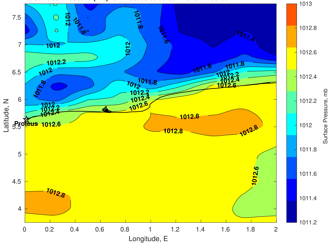
Surface Pressure (mb) for Proteus at 03-Jan-2026 12:00:00
