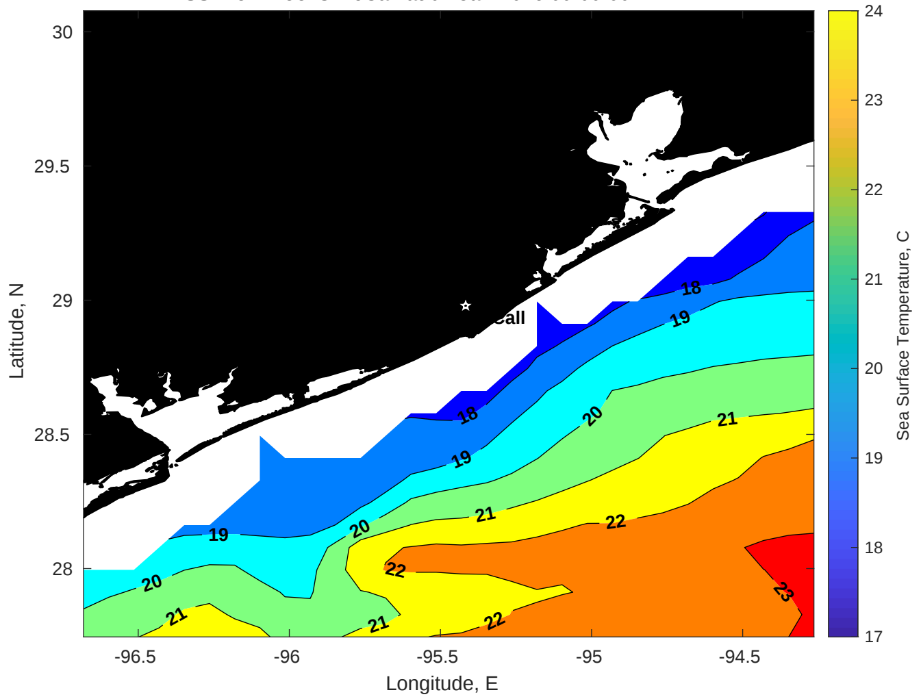
SST for Brooks McCall at 02-Jan-2026 00:00:00
