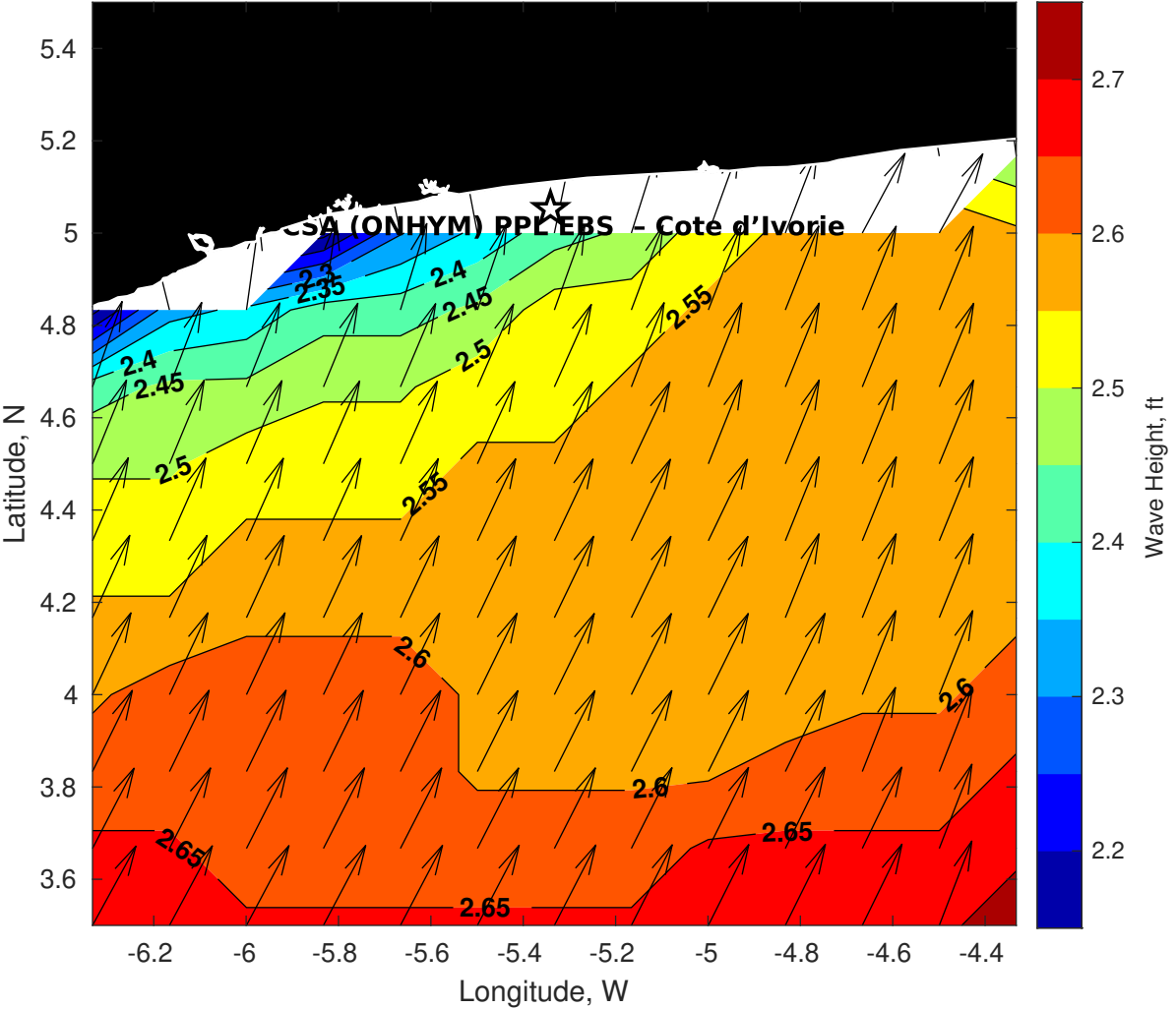
GFS Wave Height (ft) for CSA (ONHYM) PPL EBS - Cote d'Ivoire at 03-Jan-2026 09:00:00
