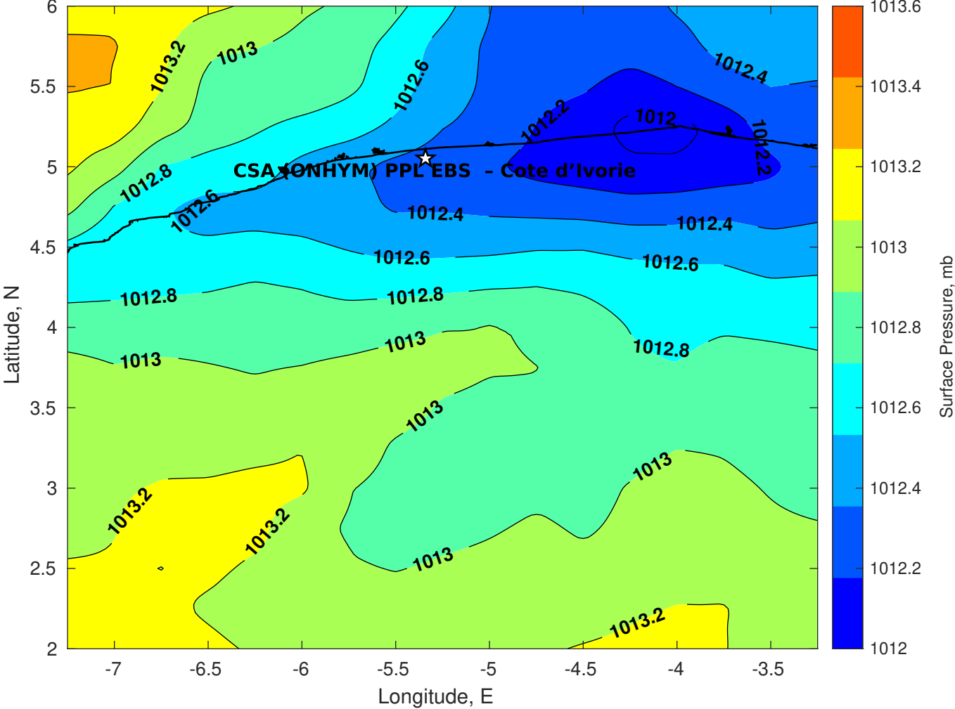
Surface Pressure (mb) for CSA (ONHYM) PPL EBS - Cote d'Ivoire at 04-Jan-2026 00:00:00
