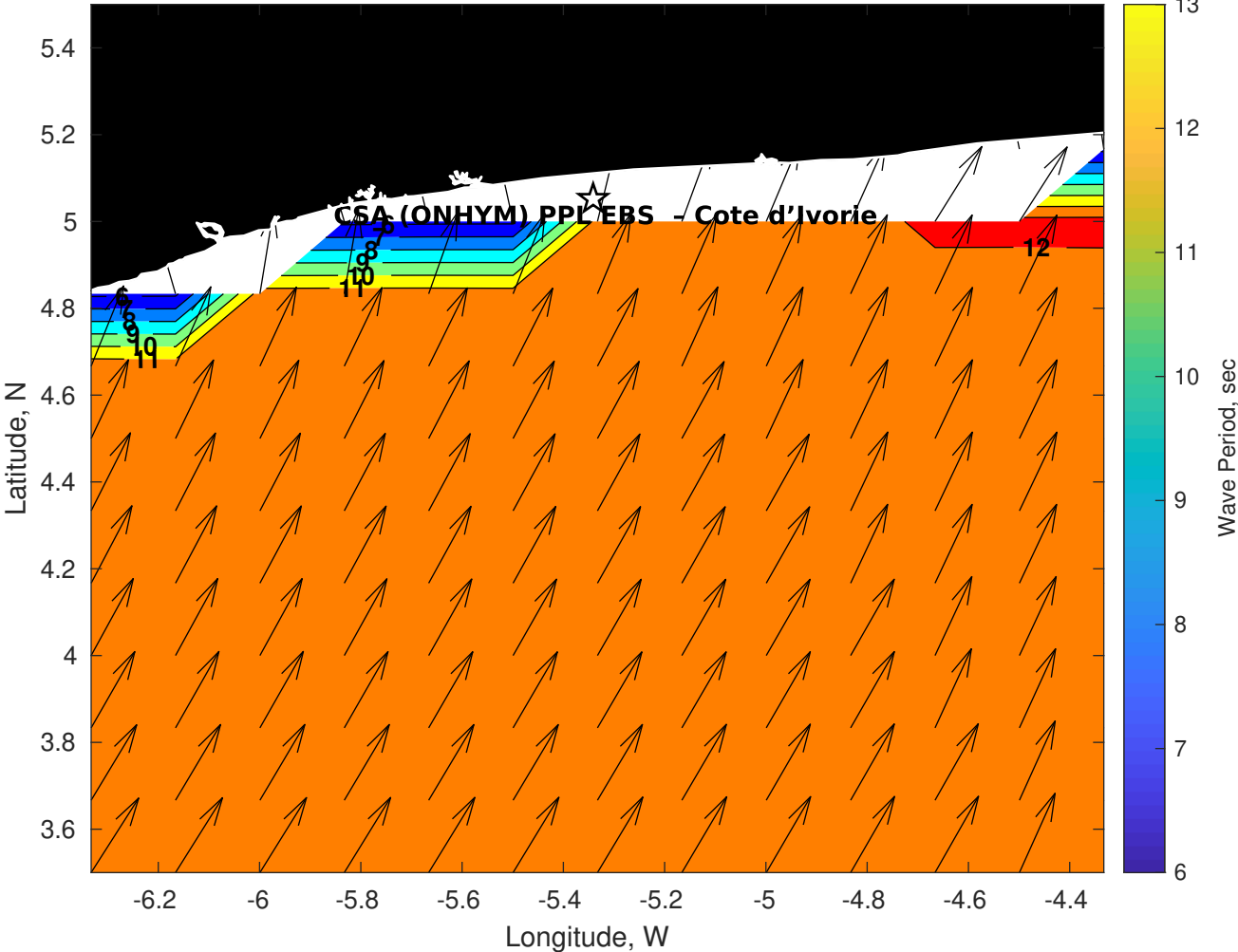
GFS Wave Period (sec) for CSA (ONHYM) PPL EBS - Cote d'Ivoire at 03-Jan-2026 09:00:00
