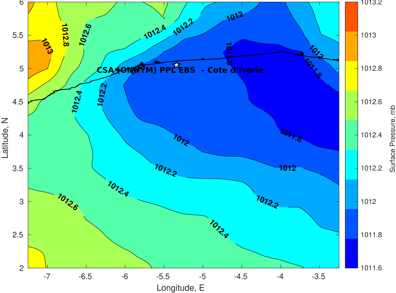
Surface Pressure (mb) for CSA (ONHYM) PPL EBS - Cote d'Ivoire at 05-Jan-2026 00:00:00
